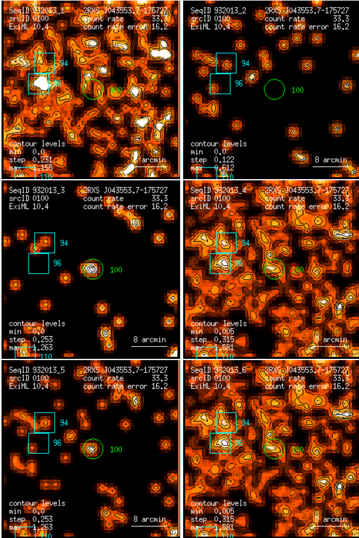
Figure 100: RASS 932013: detection 0100: band rate images, Gaussian filter: (1) PSPC channels 11 – 41, (2) 52 – 90, (3) 91 – 201, (4) 11 – 235, (5) 52 – 201, (6) 11 – 201. Broad band rates in counts/ks. Band rate contour levels in counts/ks/arcmin 2 .
