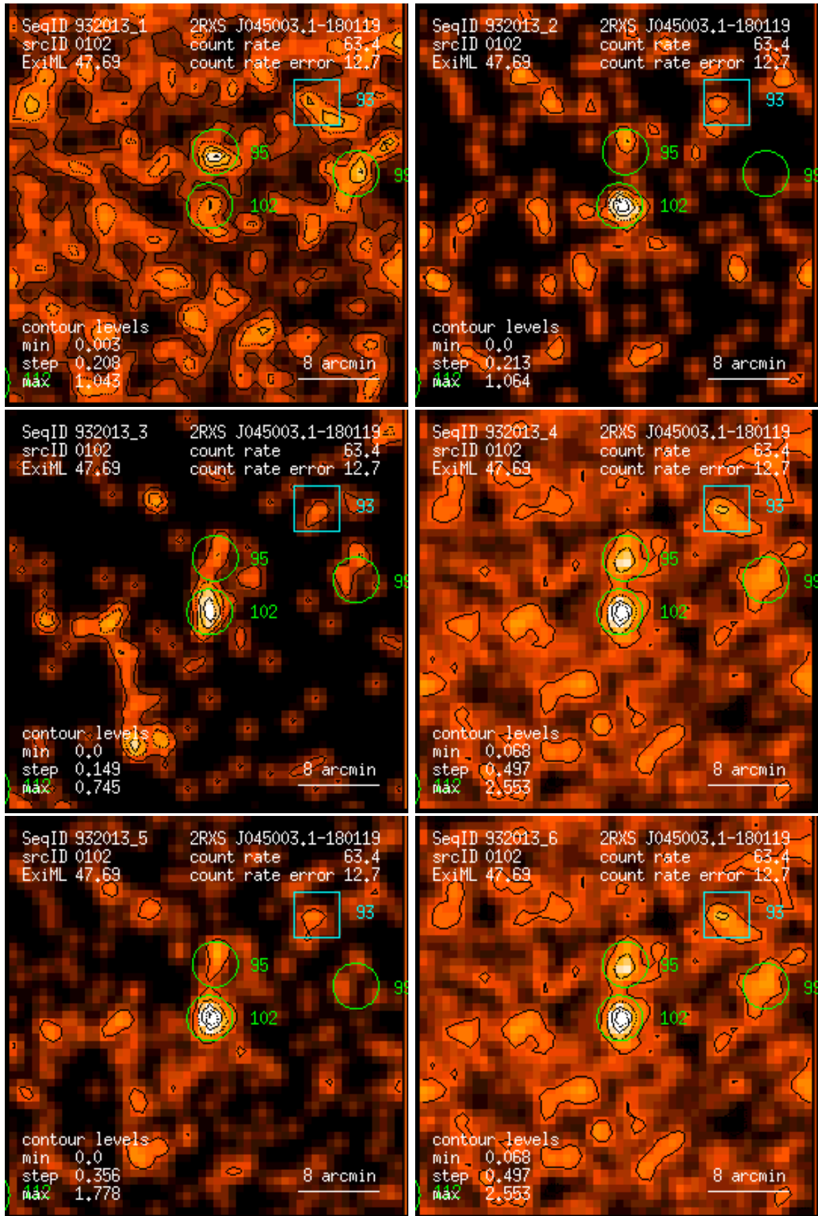
Figure 102: RASS 932013: detection 0102: band rate images, Gaussian filter: (1) PSPC channels 11 – 41, (2) 52 – 90, (3) 91 – 201, (4) 11 – 235, (5) 52 – 201, (6) 11 – 201. Broad band rates in counts/ks. Band rate contour levels in counts/ks/arcmin 2 .
