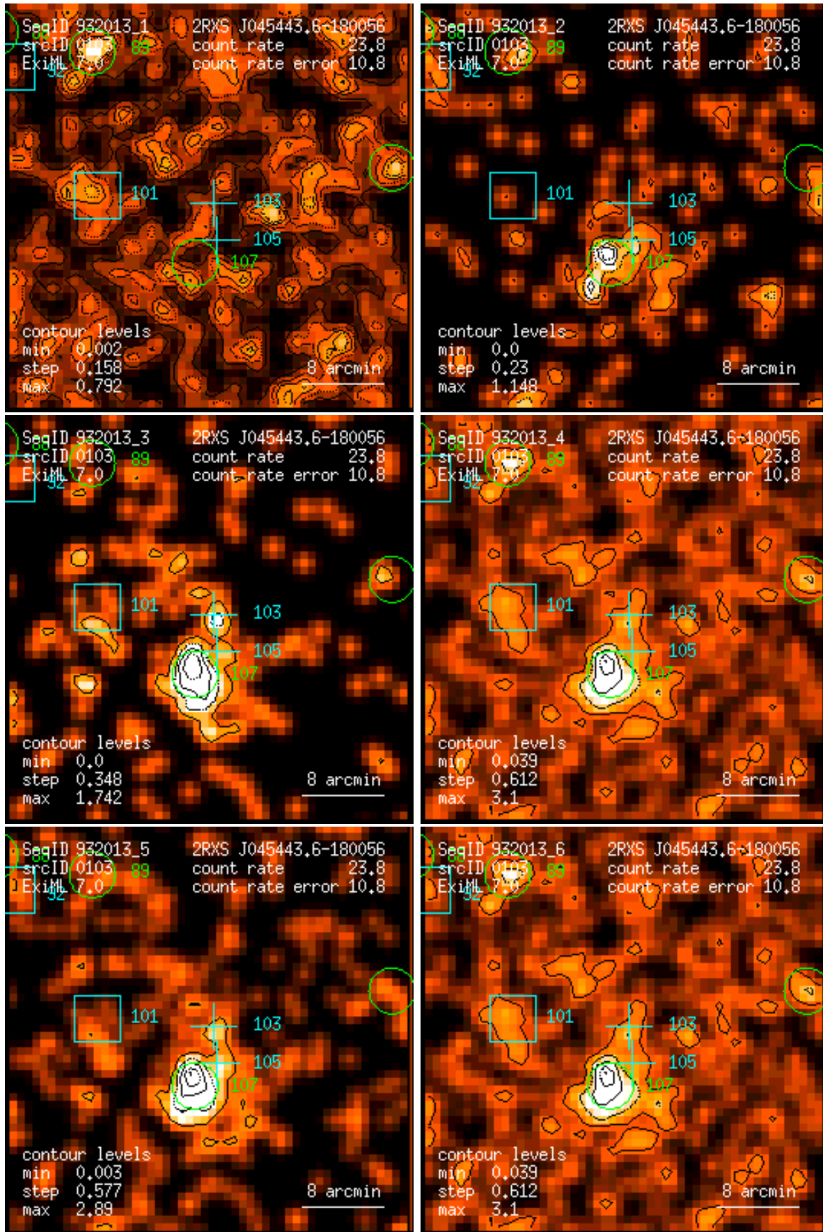
Figure 103: RASS 932013: detection 0103: band rate images, Gaussian filter: (1) PSPC channels 11 – 41, (2) 52 – 90, (3) 91 – 201, (4) 11 – 235, (5) 52 – 201, (6) 11 – 201. Broad band rates in counts/ks. Band rate contour levels in counts/ks/arcmin 2 .
