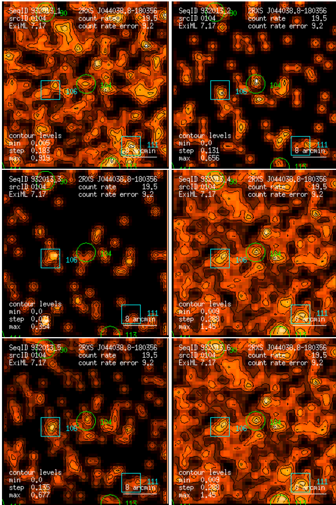
Figure 104: RASS 932013: detection 0104: band rate images, Gaussian filter: (1) PSPC channels 11 – 41, (2) 52 – 90, (3) 91 – 201, (4) 11 – 235, (5) 52 – 201, (6) 11 – 201. Broad band rates in counts/ks. Band rate contour levels in counts/ks/arcmin 2 .
