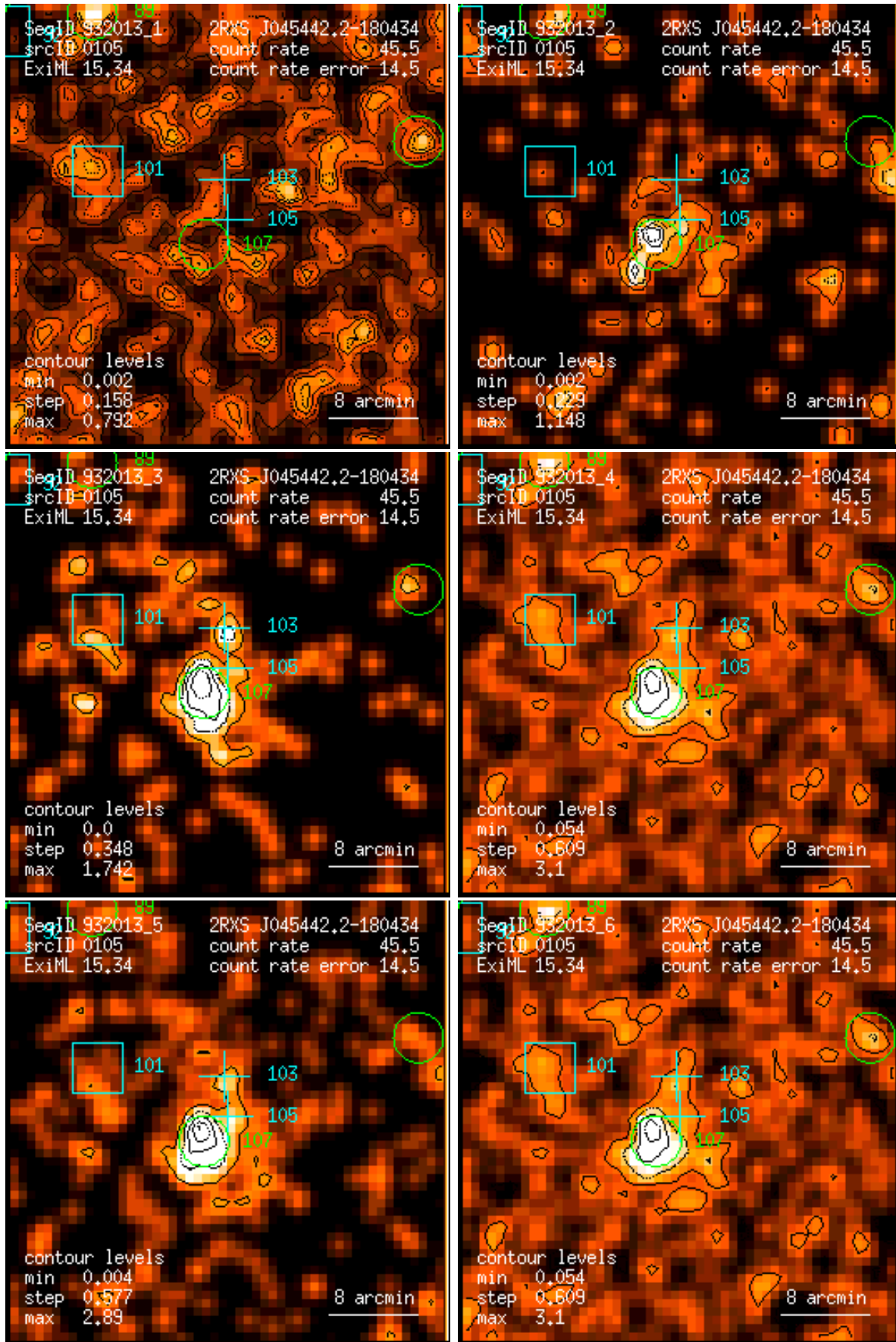
Figure 105: RASS 932013: detection 0105: band rate images, Gaussian filter: (1) PSPC channels 11 – 41, (2) 52 – 90, (3) 91 – 201, (4) 11 – 235, (5) 52 – 201, (6) 11 – 201. Broad band rates in counts/ks. Band rate contour levels in counts/ks/arcmin 2 .
