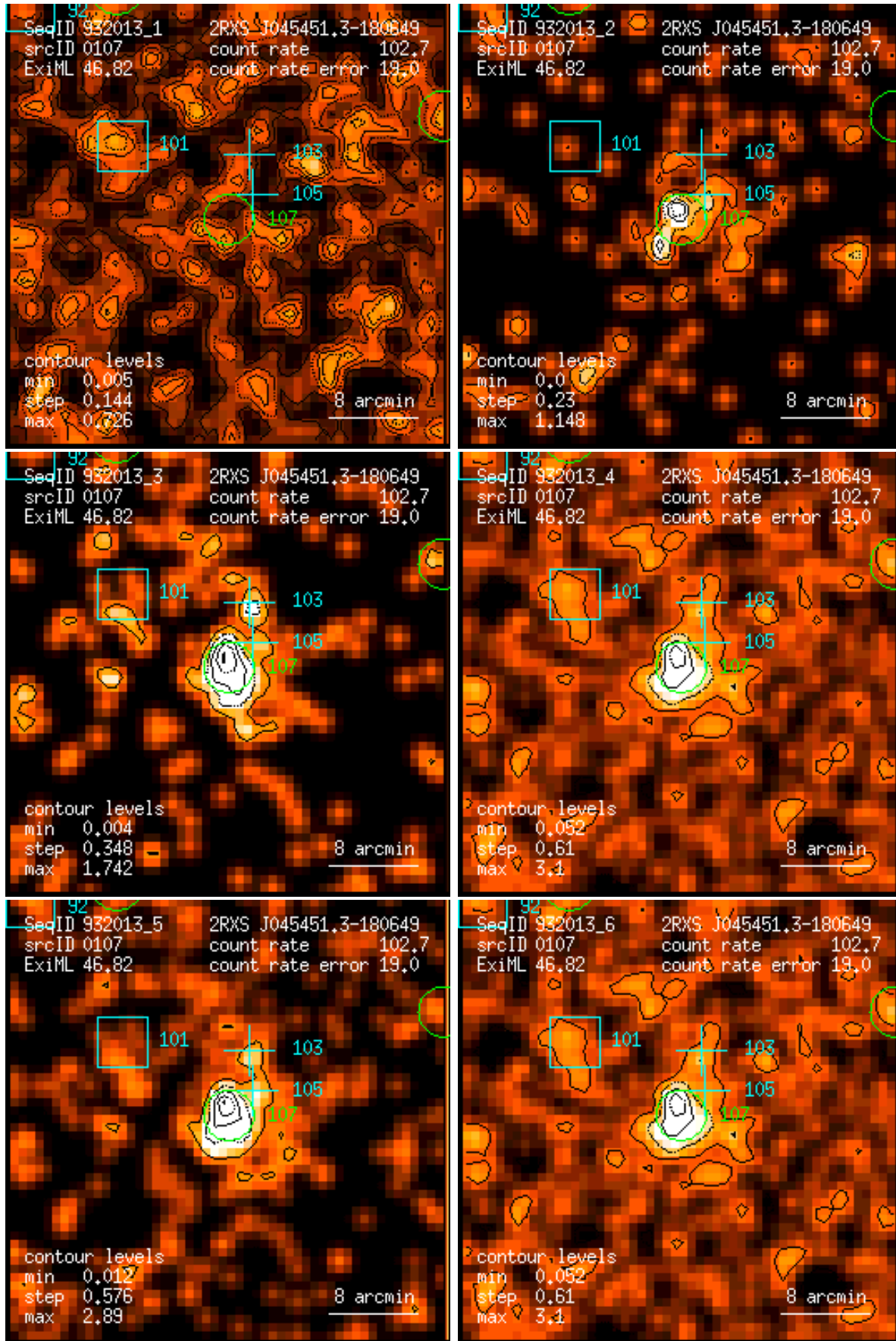
Figure 107: RASS 932013: detection 0107: band rate images, Gaussian filter: (1) PSPC channels 11 – 41, (2) 52 – 90, (3) 91 – 201, (4) 11 – 235, (5) 52 – 201, (6) 11 – 201. Broad band rates in counts/ks. Band rate contour levels in counts/ks/arcmin 2 .
