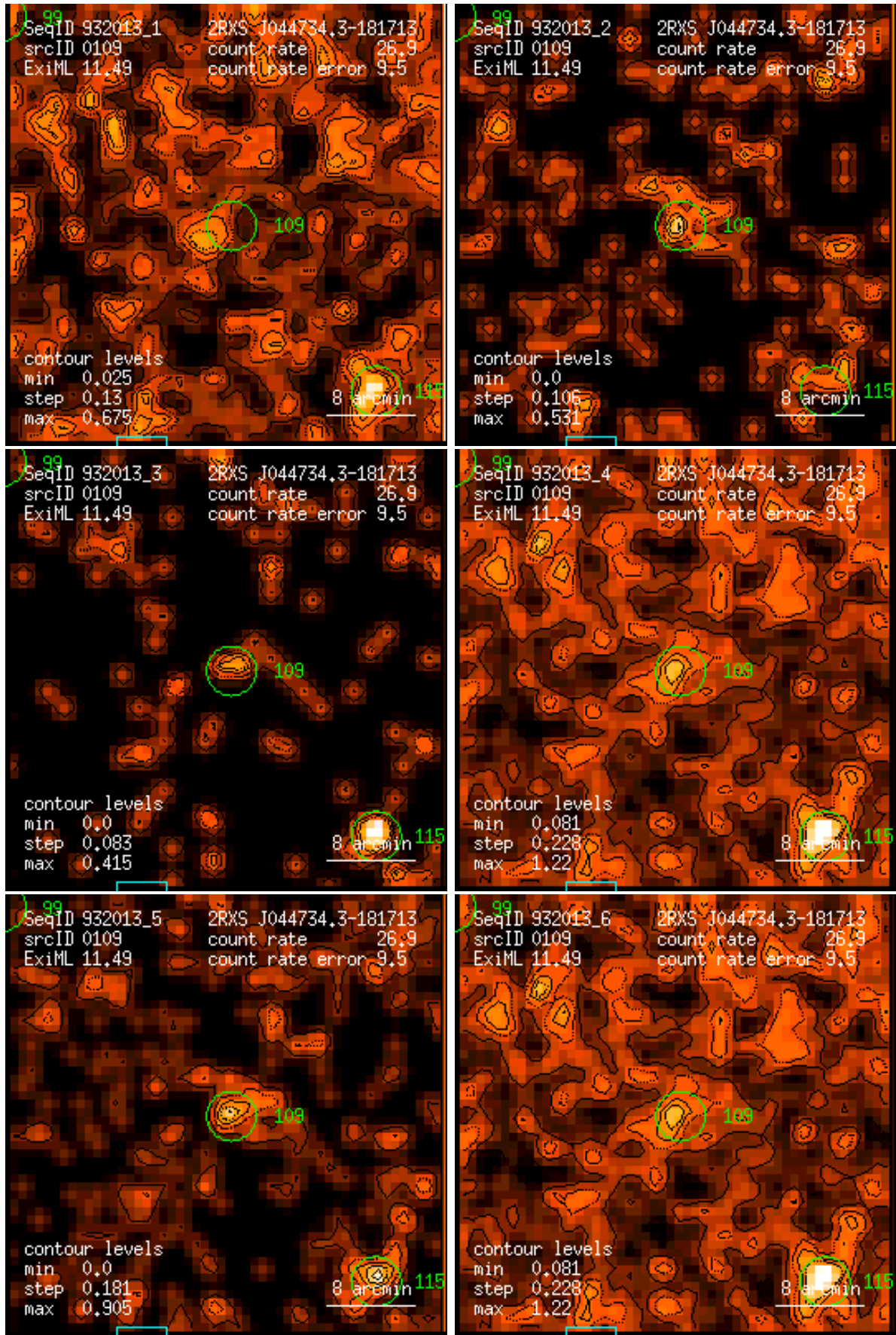
Figure 109: RASS 932013: detection 0109: band rate images, Gaussian filter: (1) PSPC channels 11 – 41, (2) 52 – 90, (3) 91 – 201, (4) 11 – 235, (5) 52 – 201, (6) 11 – 201. Broad band rates in counts/ks. Band rate contour levels in counts/ks/arcmin 2 .
