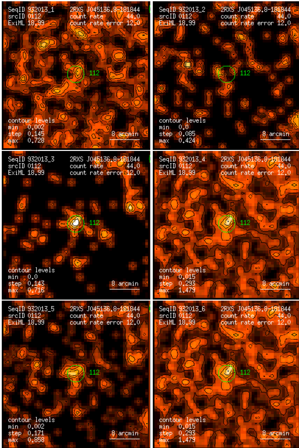
Figure 112: RASS 932013: detection 0112: band rate images, Gaussian filter: (1) PSPC channels 11 – 41, (2) 52 – 90, (3) 91 – 201, (4) 11 – 235, (5) 52 – 201, (6) 11 – 201. Broad band rates in counts/ks. Band rate contour levels in counts/ks/arcmin 2 .
