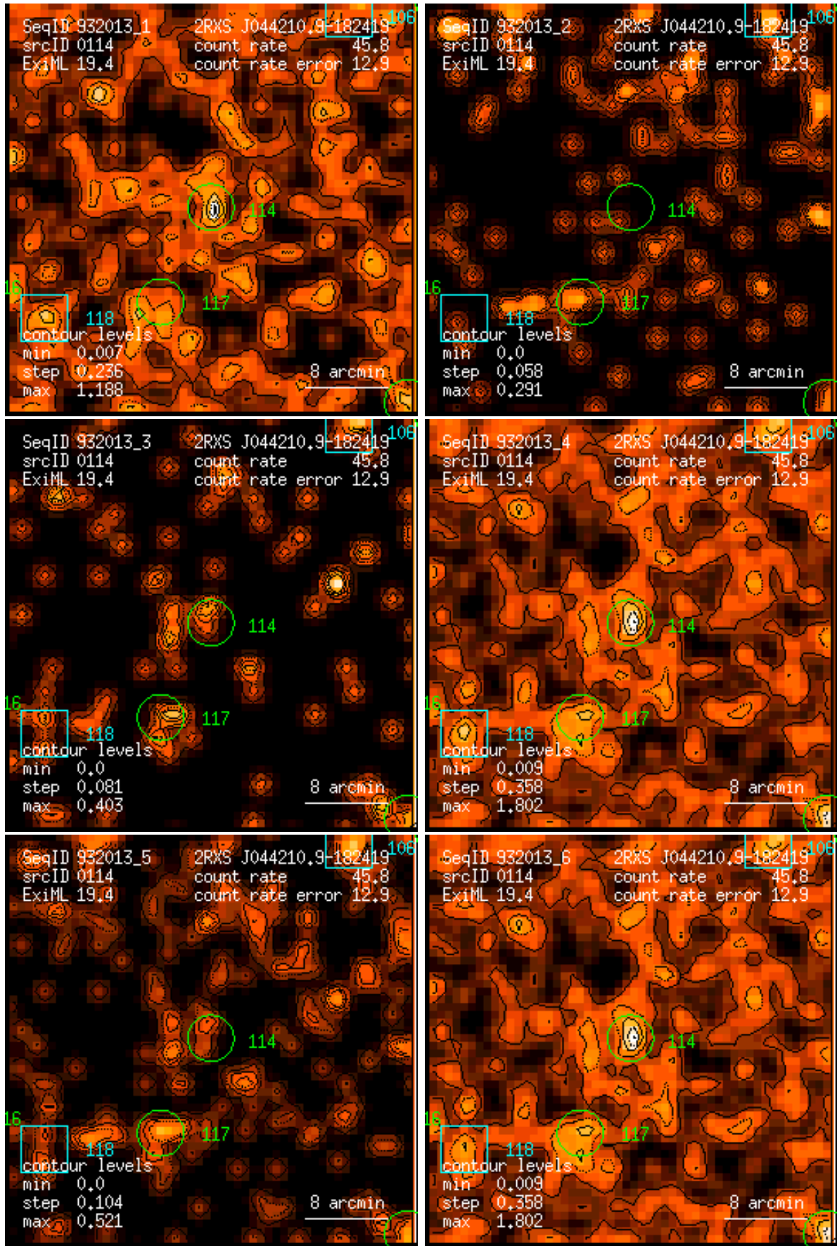
Figure 114: RASS 932013: detection 0114: band rate images, Gaussian filter: (1) PSPC channels 11 – 41, (2) 52 – 90, (3) 91 – 201, (4) 11 – 235, (5) 52 – 201, (6) 11 – 201. Broad band rates in counts/ks. Band rate contour levels in counts/ks/arcmin 2 .
