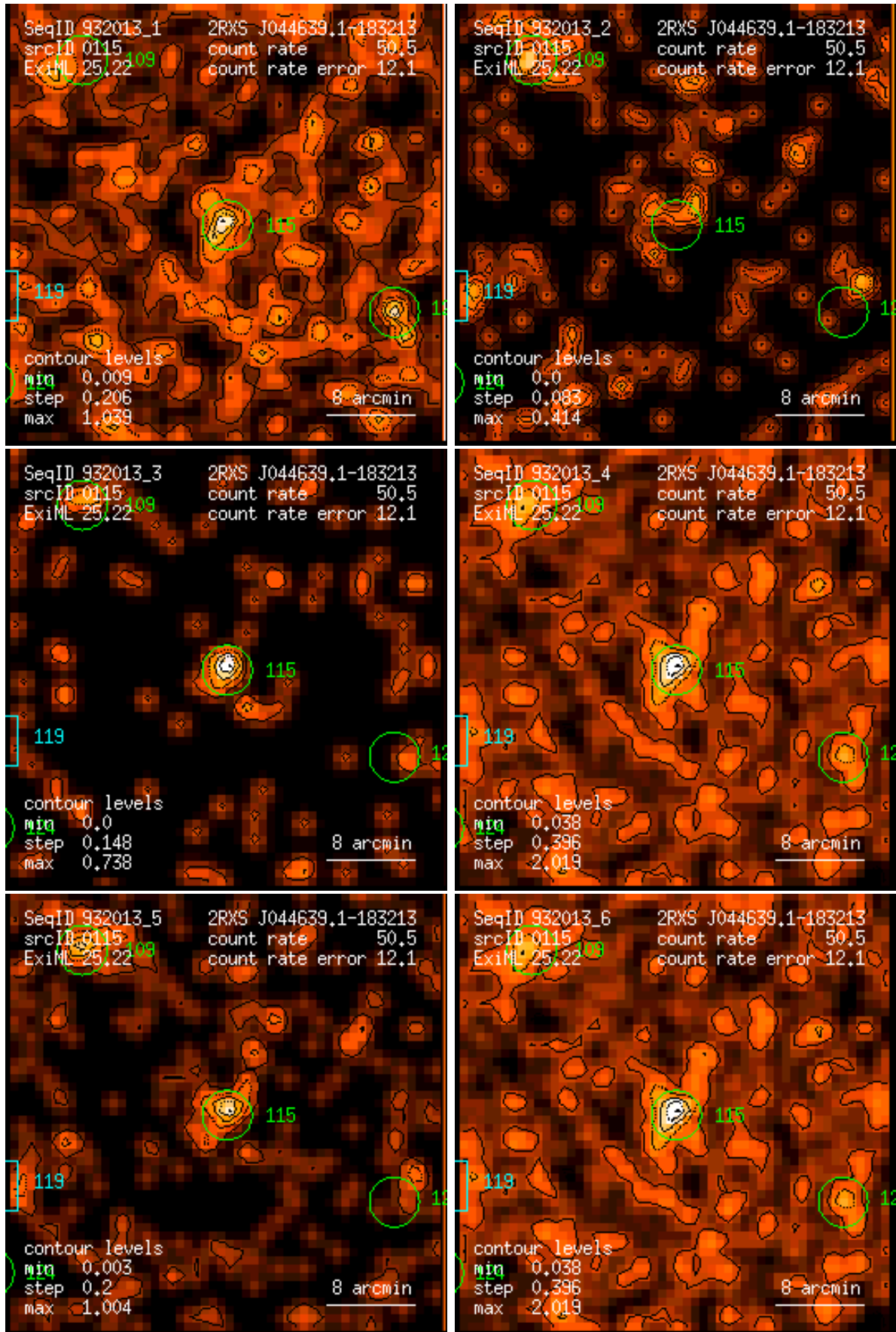
Figure 115: RASS 932013: detection 0115: band rate images, Gaussian filter: (1) PSPC channels 11 – 41, (2) 52 – 90, (3) 91 – 201, (4) 11 – 235, (5) 52 – 201, (6) 11 – 201. Broad band rates in counts/ks. Band rate contour levels in counts/ks/arcmin 2 .
