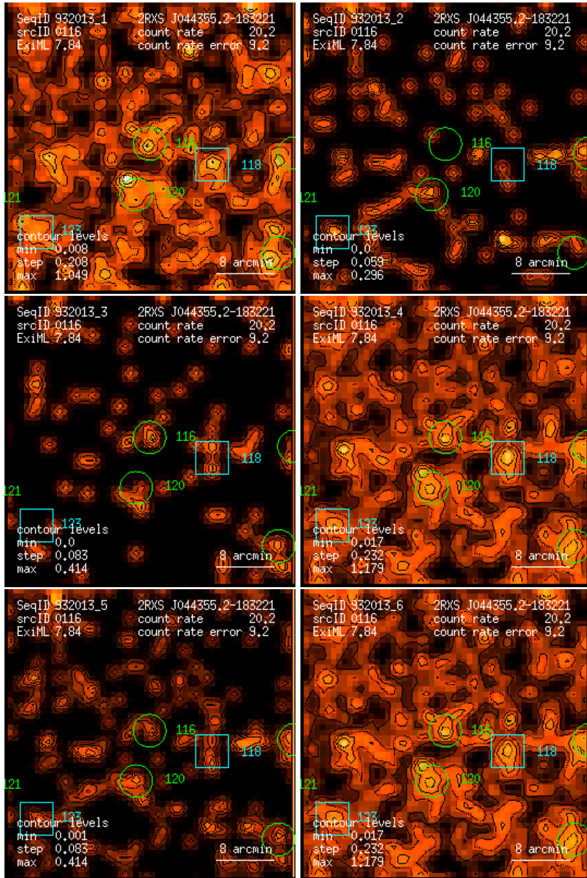
Figure 116: RASS 932013: detection 0116: band rate images, Gaussian filter: (1) PSPC channels 11 – 41, (2) 52 – 90, (3) 91 – 201, (4) 11 – 235, (5) 52 – 201, (6) 11 – 201. Broad band rates in counts/ks. Band rate contour levels in counts/ks/arcmin 2 .
