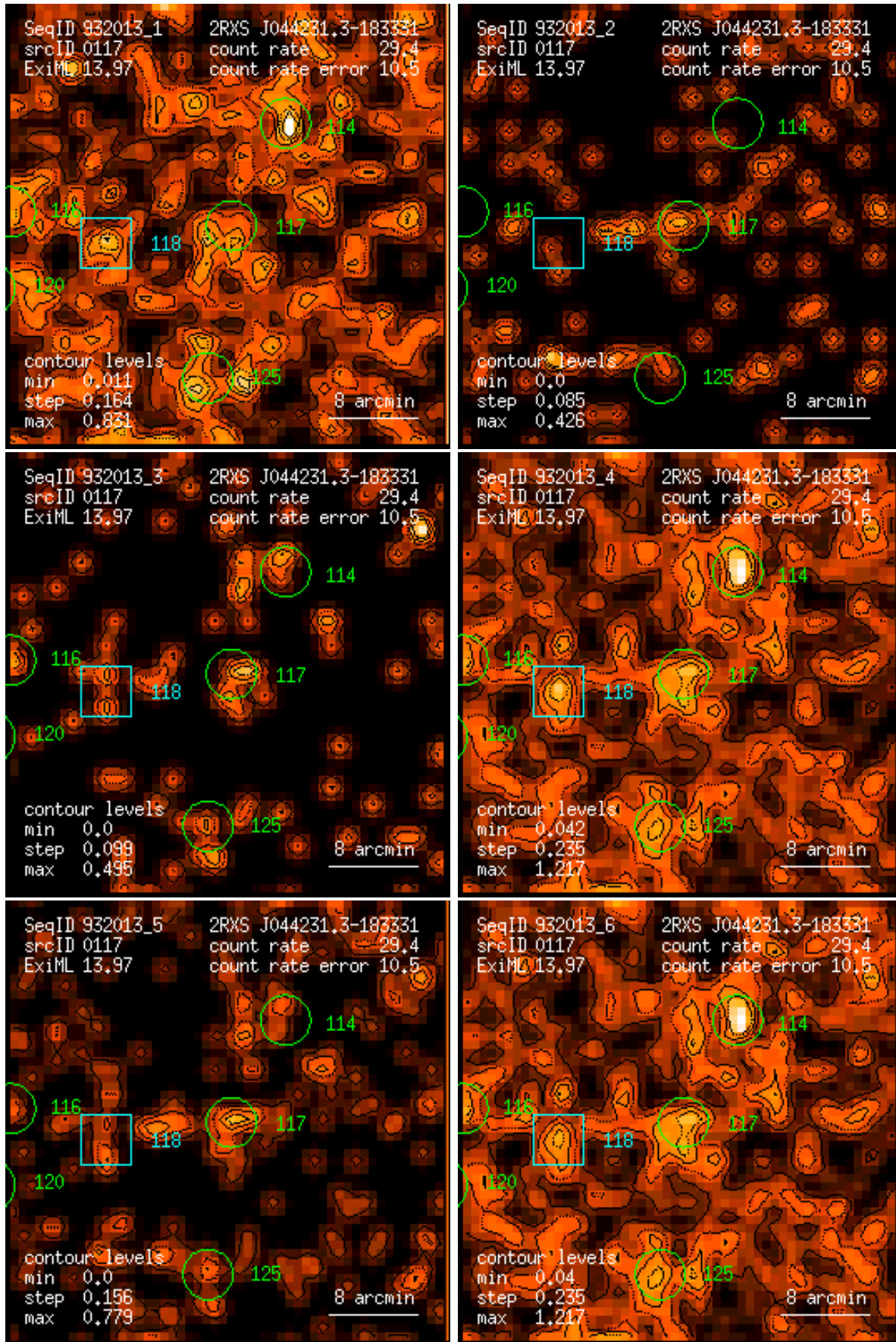
Figure 117: RASS 932013: detection 0117: band rate images, Gaussian filter: (1) PSPC channels 11 – 41, (2) 52 – 90, (3) 91 – 201, (4) 11 – 235, (5) 52 – 201, (6) 11 – 201. Broad band rates in counts/ks. Band rate contour levels in counts/ks/arcmin 2 .
