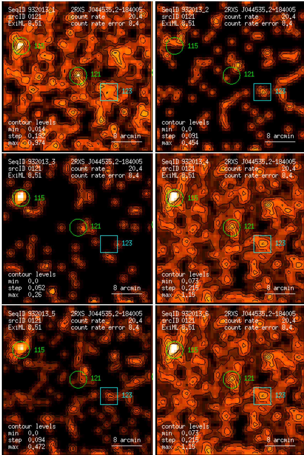
Figure 121: RASS 932013: detection 0121: band rate images, Gaussian filter: (1) PSPC channels 11 – 41, (2) 52 – 90, (3) 91 – 201, (4) 11 – 235, (5) 52 – 201, (6) 11 – 201. Broad band rates in counts/ks. Band rate contour levels in counts/ks/arcmin 2 .
