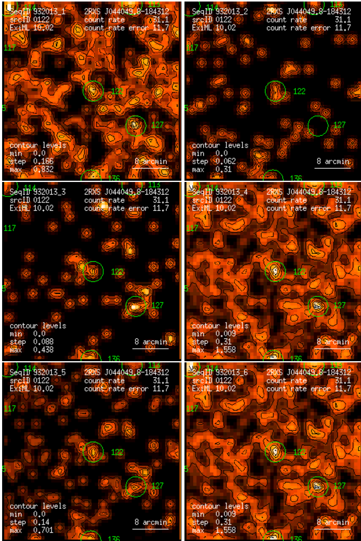
Figure 122: RASS 932013: detection 0122: band rate images, Gaussian filter: (1) PSPC channels 11 – 41, (2) 52 – 90, (3) 91 – 201, (4) 11 – 235, (5) 52 – 201, (6) 11 – 201. Broad band rates in counts/ks. Band rate contour levels in counts/ks/arcmin 2 .
