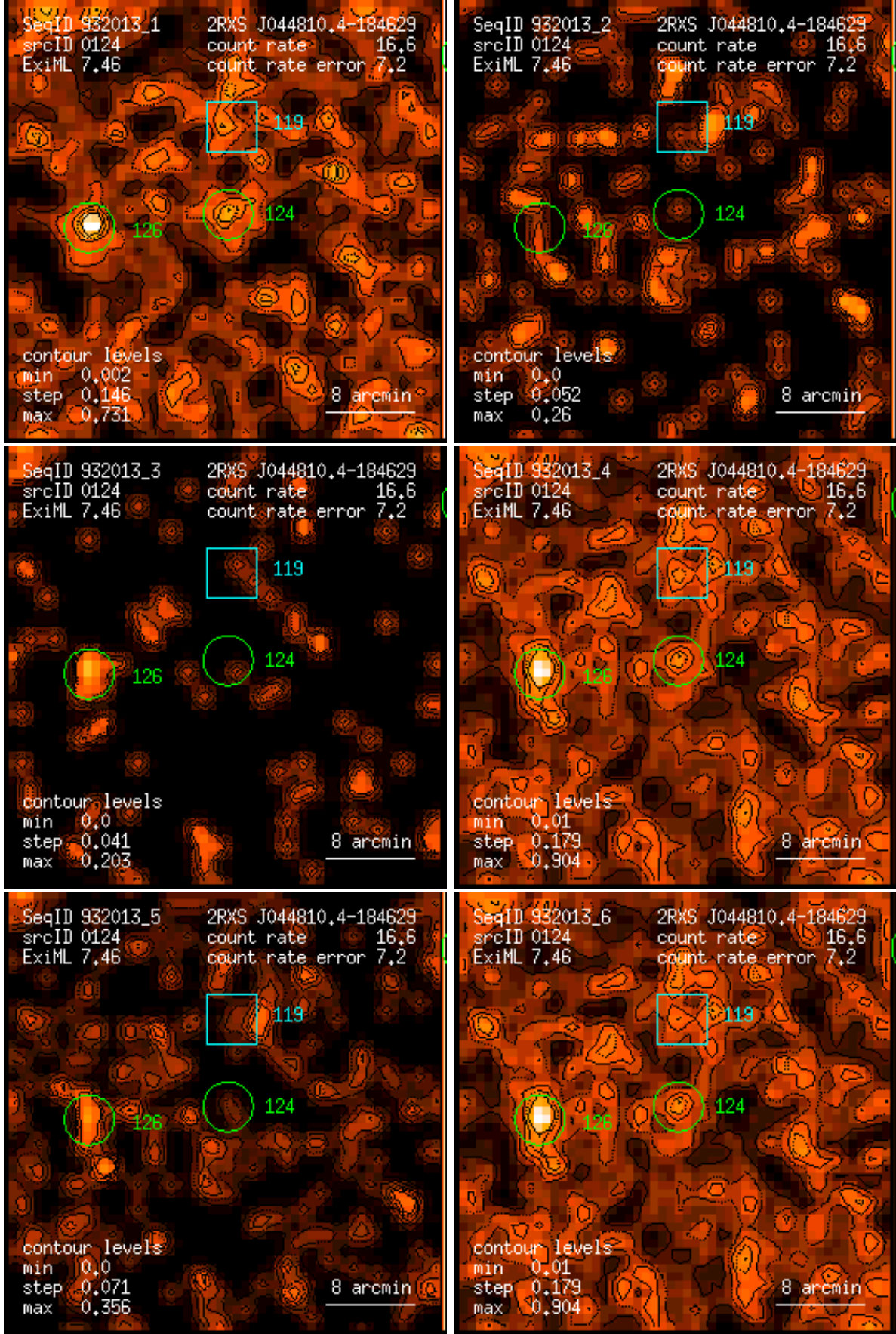
Figure 124: RASS 932013: detection 0124: band rate images, Gaussian filter: (1) PSPC channels 11 – 41, (2) 52 – 90, (3) 91 – 201, (4) 11 – 235, (5) 52 – 201, (6) 11 – 201. Broad band rates in counts/ks. Band rate contour levels in counts/ks/arcmin 2 .
