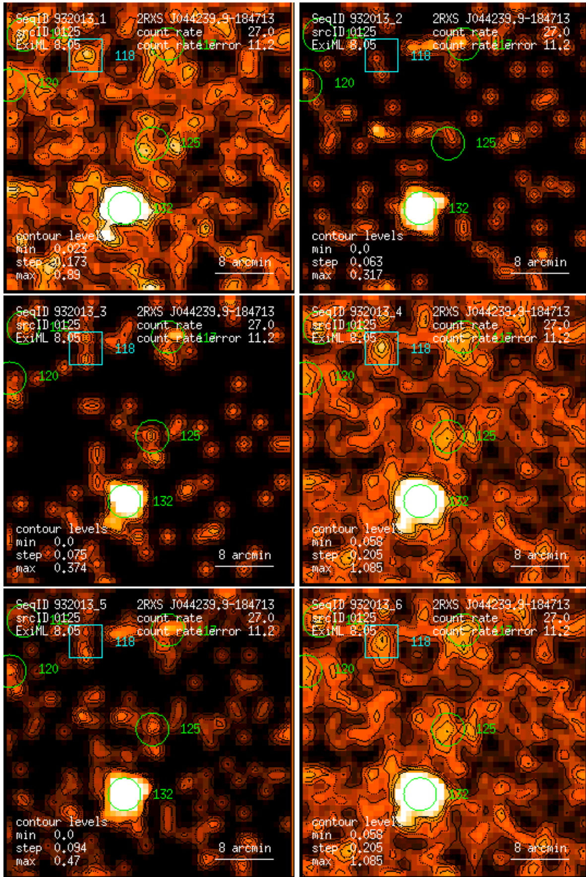
Figure 125: RASS 932013: detection 0125: band rate images, Gaussian filter: (1) PSPC channels 11 – 41, (2) 52 – 90, (3) 91 – 201, (4) 11 – 235, (5) 52 – 201, (6) 11 – 201. Broad band rates in counts/ks. Band rate contour levels in counts/ks/arcmin 2 .
