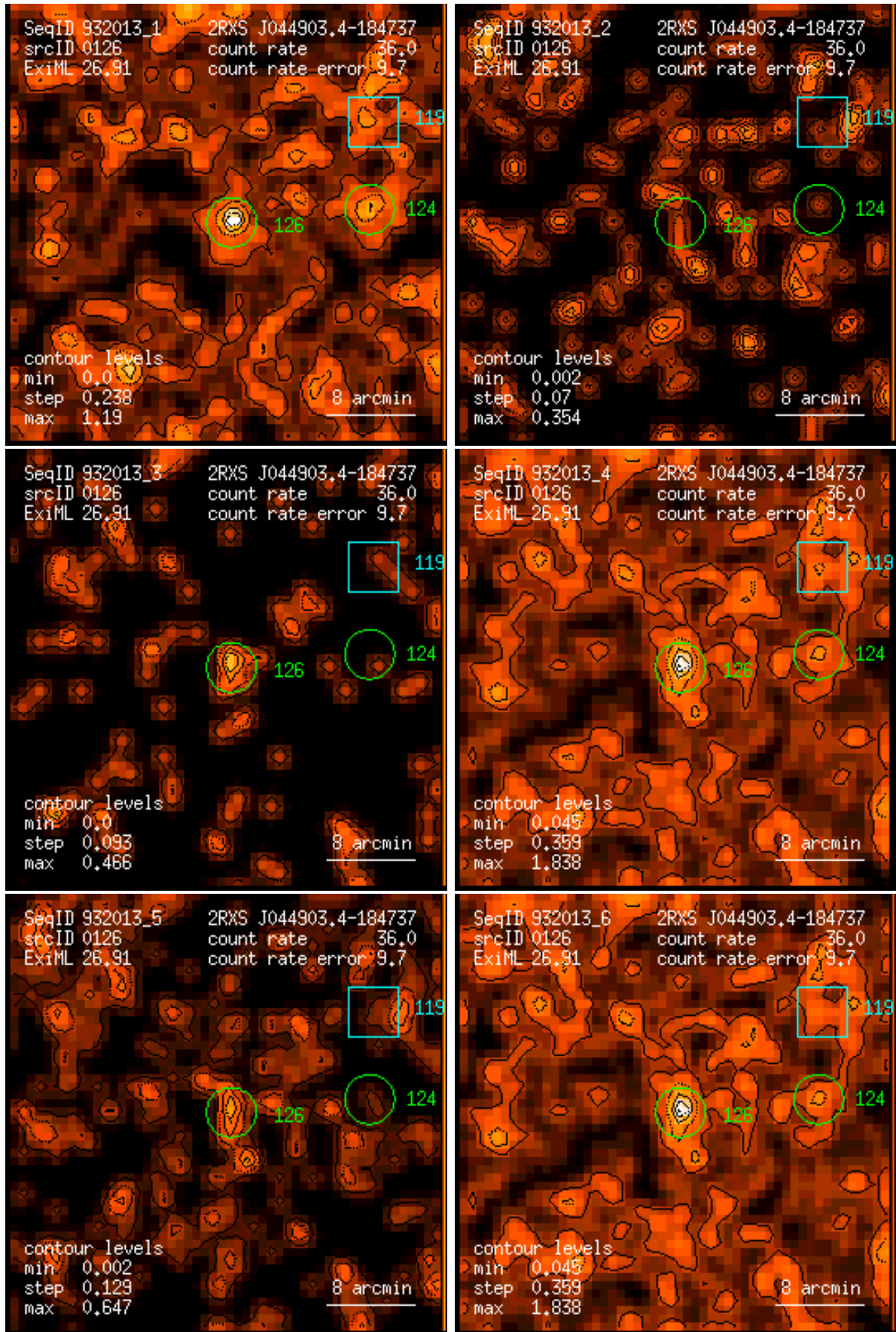
Figure 126: RASS 932013: detection 0126: band rate images, Gaussian filter: (1) PSPC channels 11 – 41, (2) 52 – 90, (3) 91 – 201, (4) 11 – 235, (5) 52 – 201, (6) 11 – 201. Broad band rates in counts/ks. Band rate contour levels in counts/ks/arcmin 2 .
