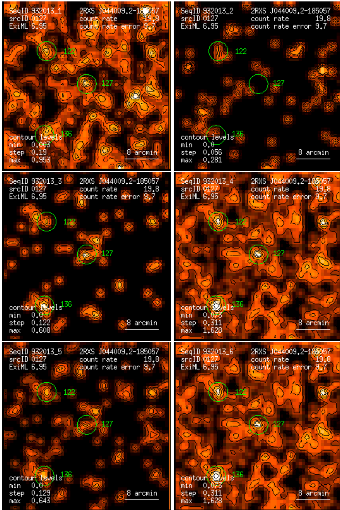
Figure 127: RASS 932013: detection 0127: band rate images, Gaussian filter: (1) PSPC channels 11 – 41, (2) 52 – 90, (3) 91 – 201, (4) 11 – 235, (5) 52 – 201, (6) 11 – 201. Broad band rates in counts/ks. Band rate contour levels in counts/ks/arcmin 2 .
