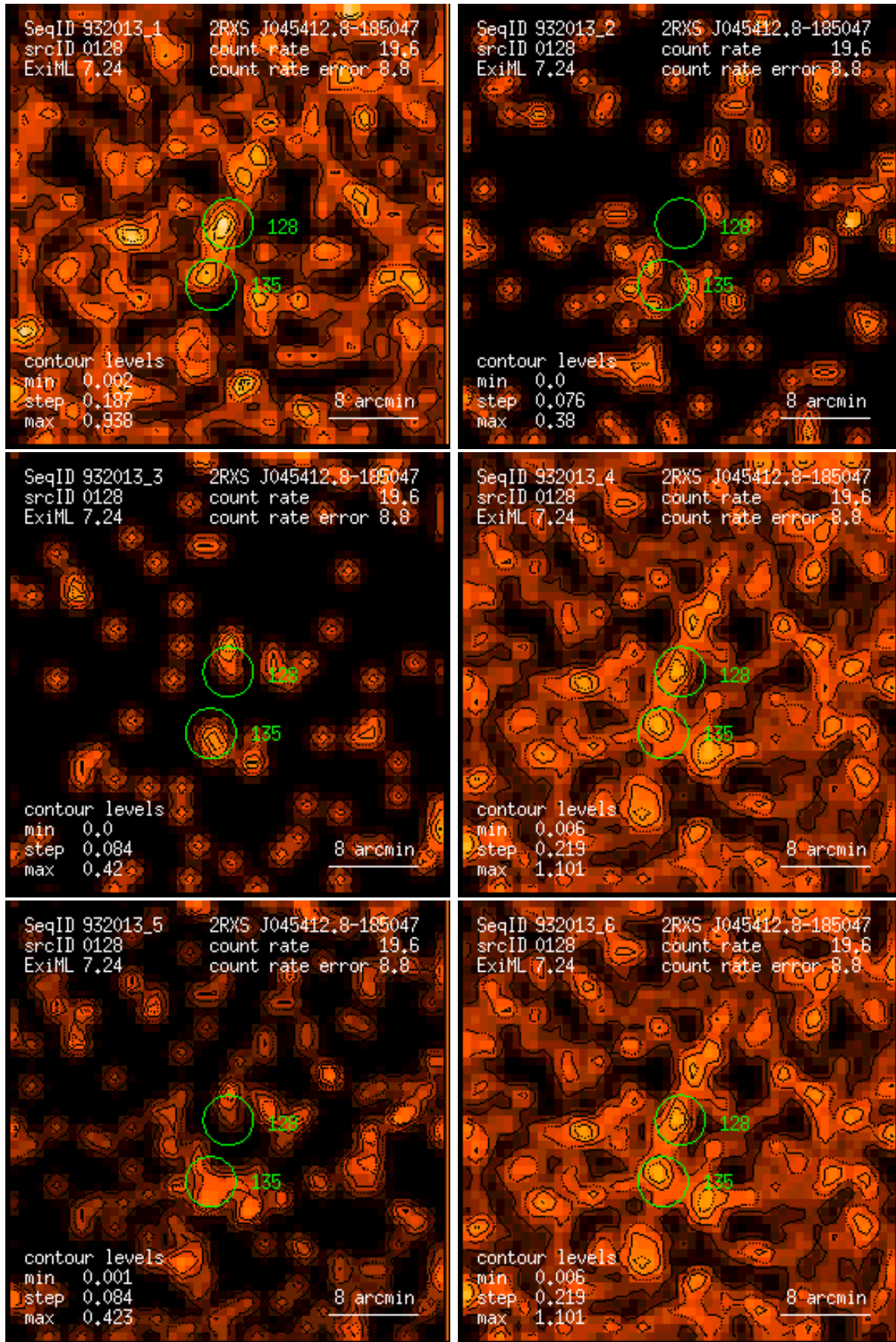
Figure 128: RASS 932013: detection 0128: band rate images, Gaussian filter: (1) PSPC channels 11 – 41, (2) 52 – 90, (3) 91 – 201, (4) 11 – 235, (5) 52 – 201, (6) 11 – 201. Broad band rates in counts/ks. Band rate contour levels in counts/ks/arcmin 2 .
