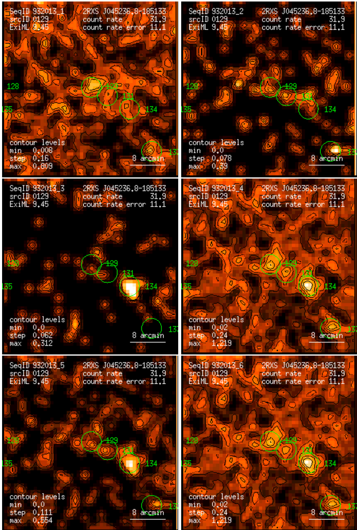
Figure 129: RASS 932013: detection 0129: band rate images, Gaussian filter: (1) PSPC channels 11 – 41, (2) 52 – 90, (3) 91 – 201, (4) 11 – 235, (5) 52 – 201, (6) 11 – 201. Broad band rates in counts/ks. Band rate contour levels in counts/ks/arcmin 2 .
