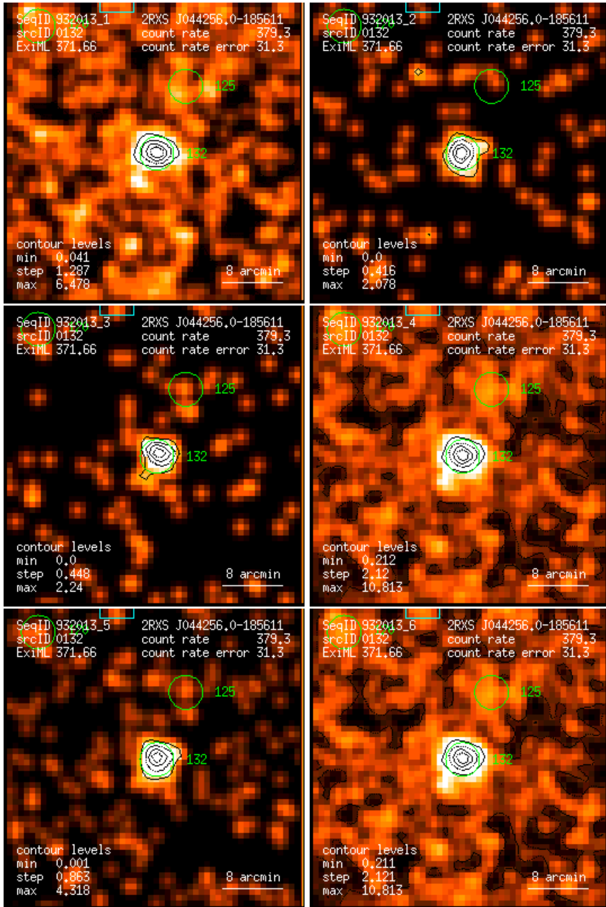
Figure 132: RASS 932013: detection 0132: band rate images, Gaussian filter: (1) PSPC channels 11 – 41, (2) 52 – 90, (3) 91 – 201, (4) 11 – 235, (5) 52 – 201, (6) 11 – 201. Broad band rates in counts/ks. Band rate contour levels in counts/ks/arcmin 2 .
