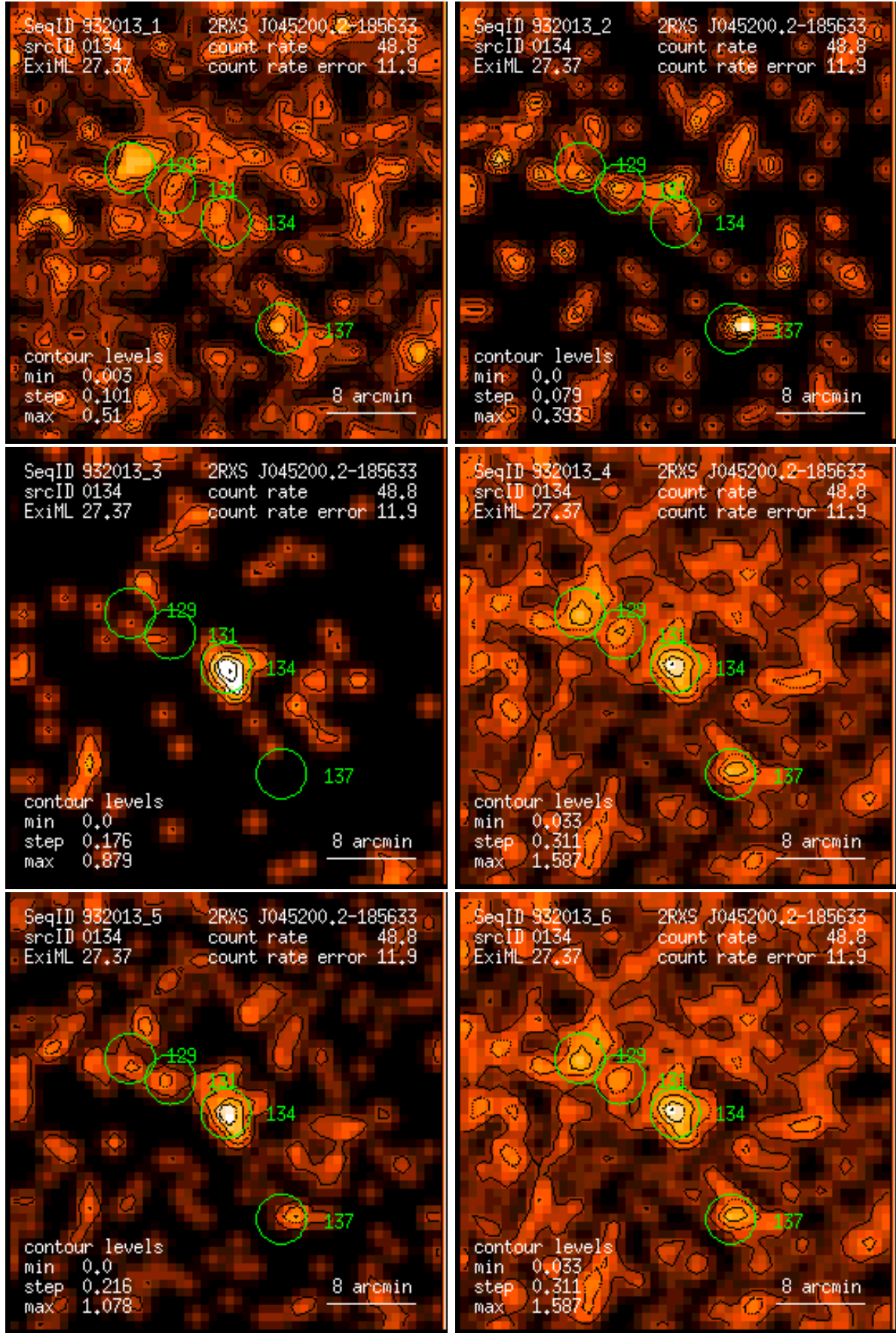
Figure 134: RASS 932013: detection 0134: band rate images, Gaussian filter: (1) PSPC channels 11 – 41, (2) 52 – 90, (3) 91 – 201, (4) 11 – 235, (5) 52 – 201, (6) 11 – 201. Broad band rates in counts/ks. Band rate contour levels in counts/ks/arcmin 2 .
