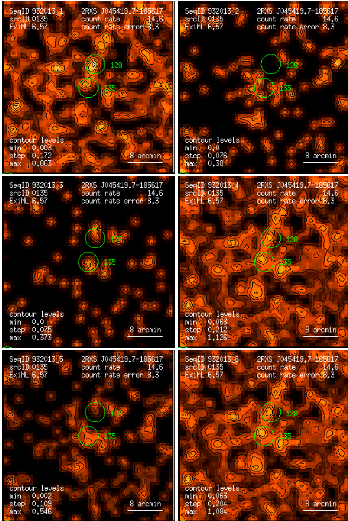
Figure 135: RASS 932013: detection 0135: band rate images, Gaussian filter: (1) PSPC channels 11 – 41, (2) 52 – 90, (3) 91 – 201, (4) 11 – 235, (5) 52 – 201, (6) 11 – 201. Broad band rates in counts/ks. Band rate contour levels in counts/ks/arcmin 2 .
