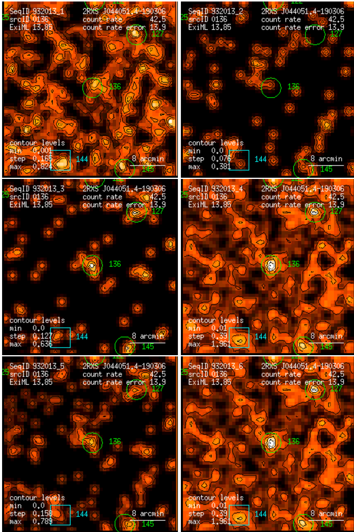
Figure 136: RASS 932013: detection 0136: band rate images, Gaussian filter: (1) PSPC channels 11 – 41, (2) 52 – 90, (3) 91 – 201, (4) 11 – 235, (5) 52 – 201, (6) 11 – 201. Broad band rates in counts/ks. Band rate contour levels in counts/ks/arcmin 2 .
