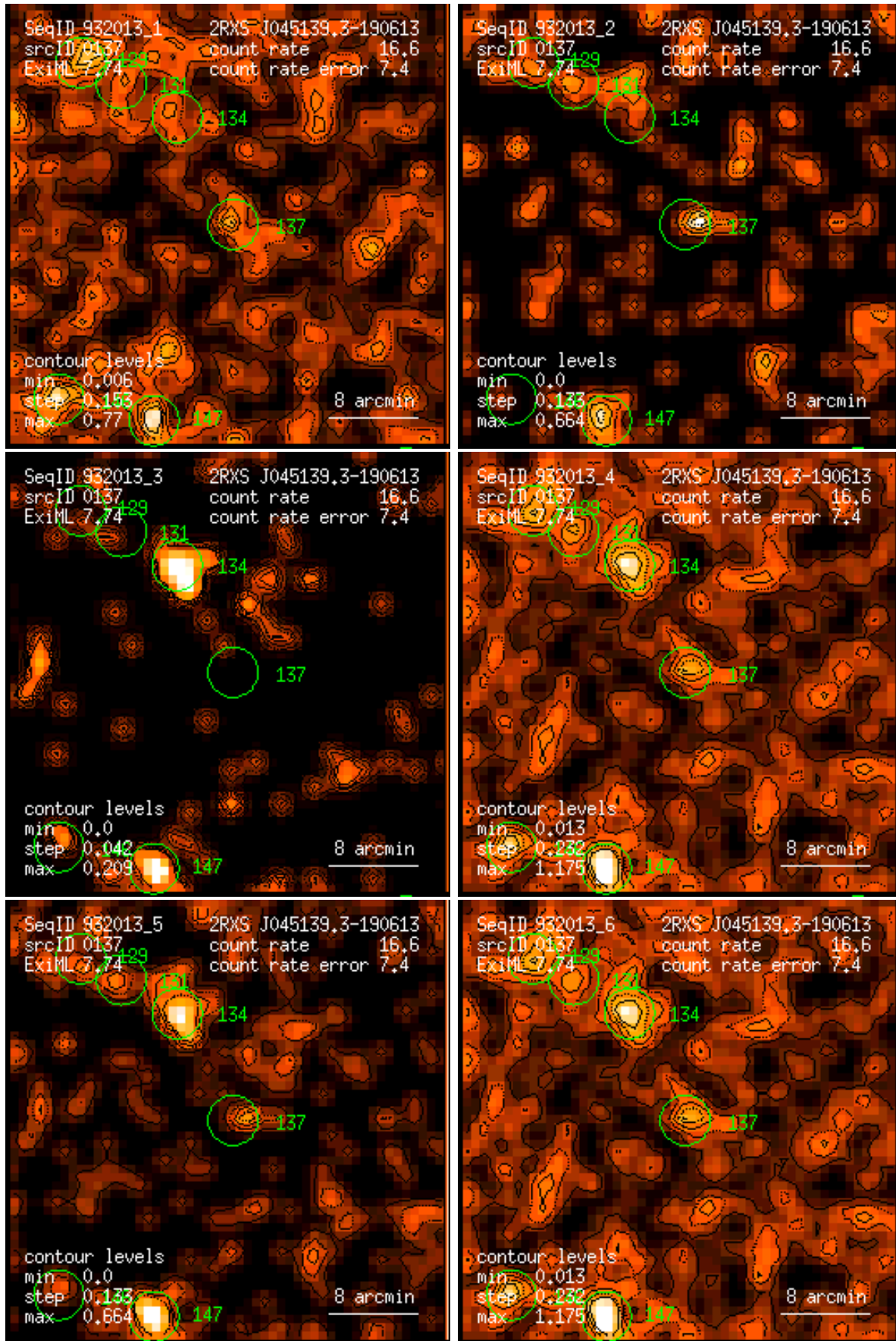
Figure 137: RASS 932013: detection 0137: band rate images, Gaussian filter: (1) PSPC channels 11 – 41, (2) 52 – 90, (3) 91 – 201, (4) 11 – 235, (5) 52 – 201, (6) 11 – 201. Broad band rates in counts/ks. Band rate contour levels in counts/ks/arcmin 2 .
