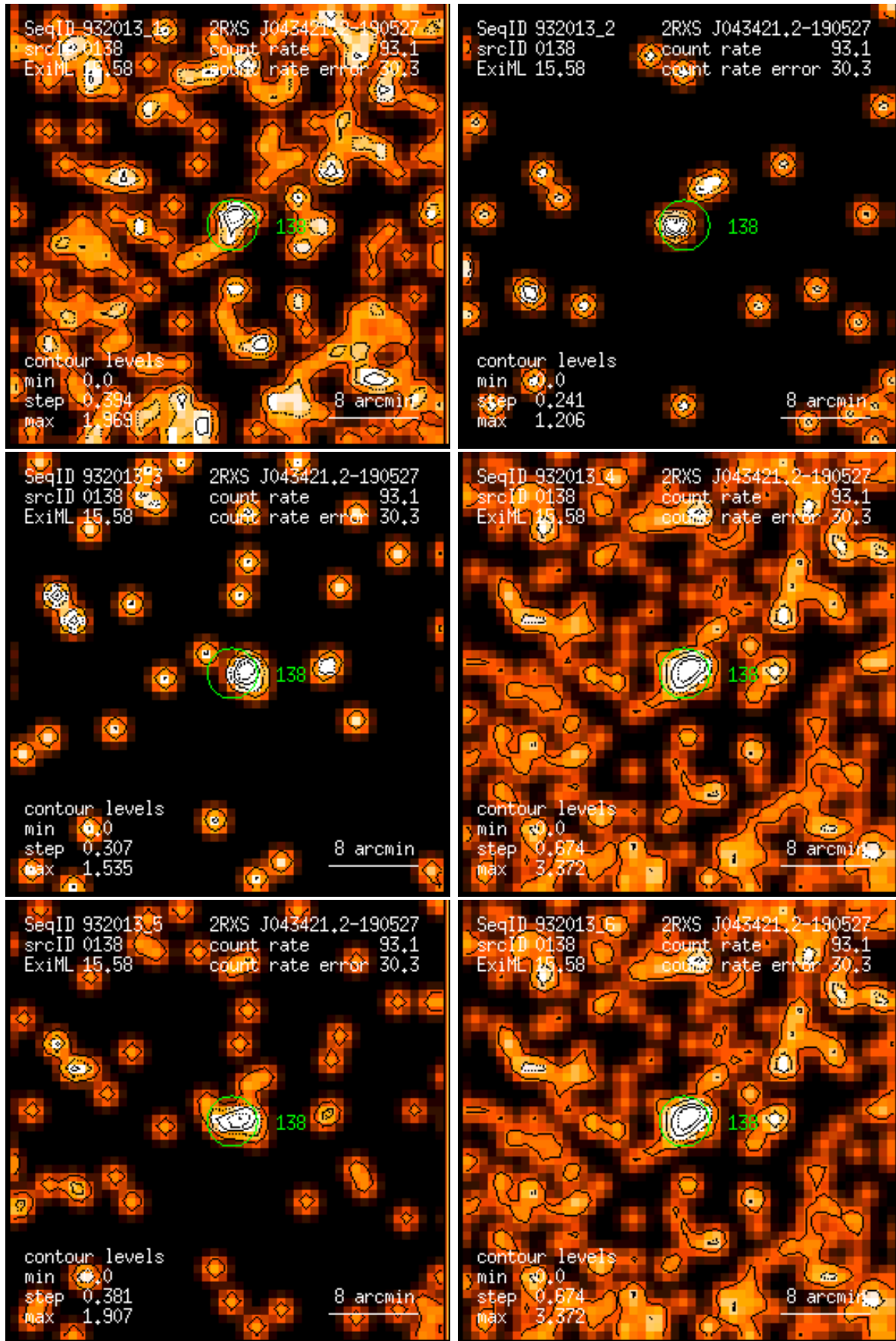
Figure 138: RASS 932013: detection 0138: band rate images, Gaussian filter: (1) PSPC channels 11 – 41, (2) 52 – 90, (3) 91 – 201, (4) 11 – 235, (5) 52 – 201, (6) 11 – 201. Broad band rates in counts/ks. Band rate contour levels in counts/ks/arcmin 2 .
