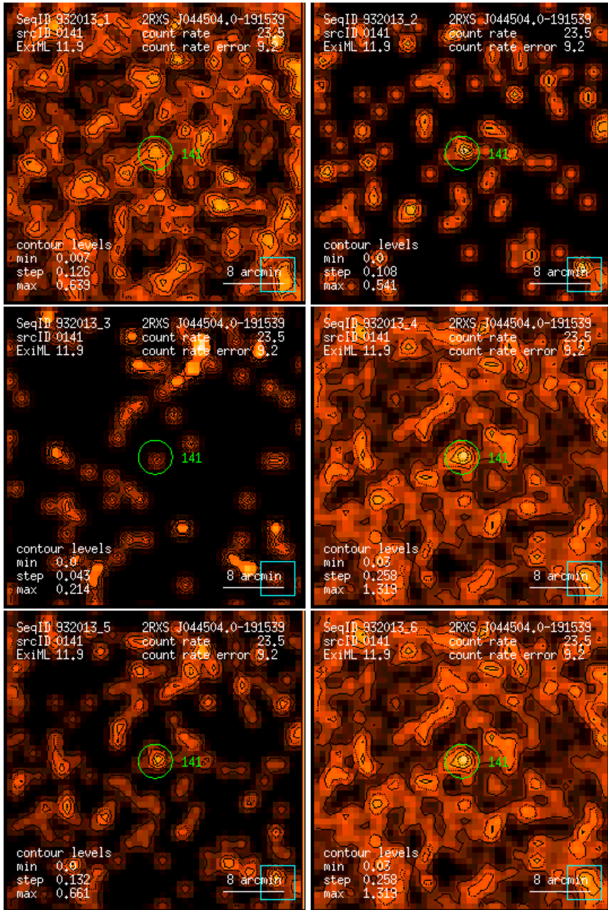
Figure 141: RASS 932013: detection 0141: band rate images, Gaussian filter: (1) PSPC channels 11 – 41, (2) 52 – 90, (3) 91 – 201, (4) 11 – 235, (5) 52 – 201, (6) 11 – 201. Broad band rates in counts/ks. Band rate contour levels in counts/ks/arcmin 2 .
