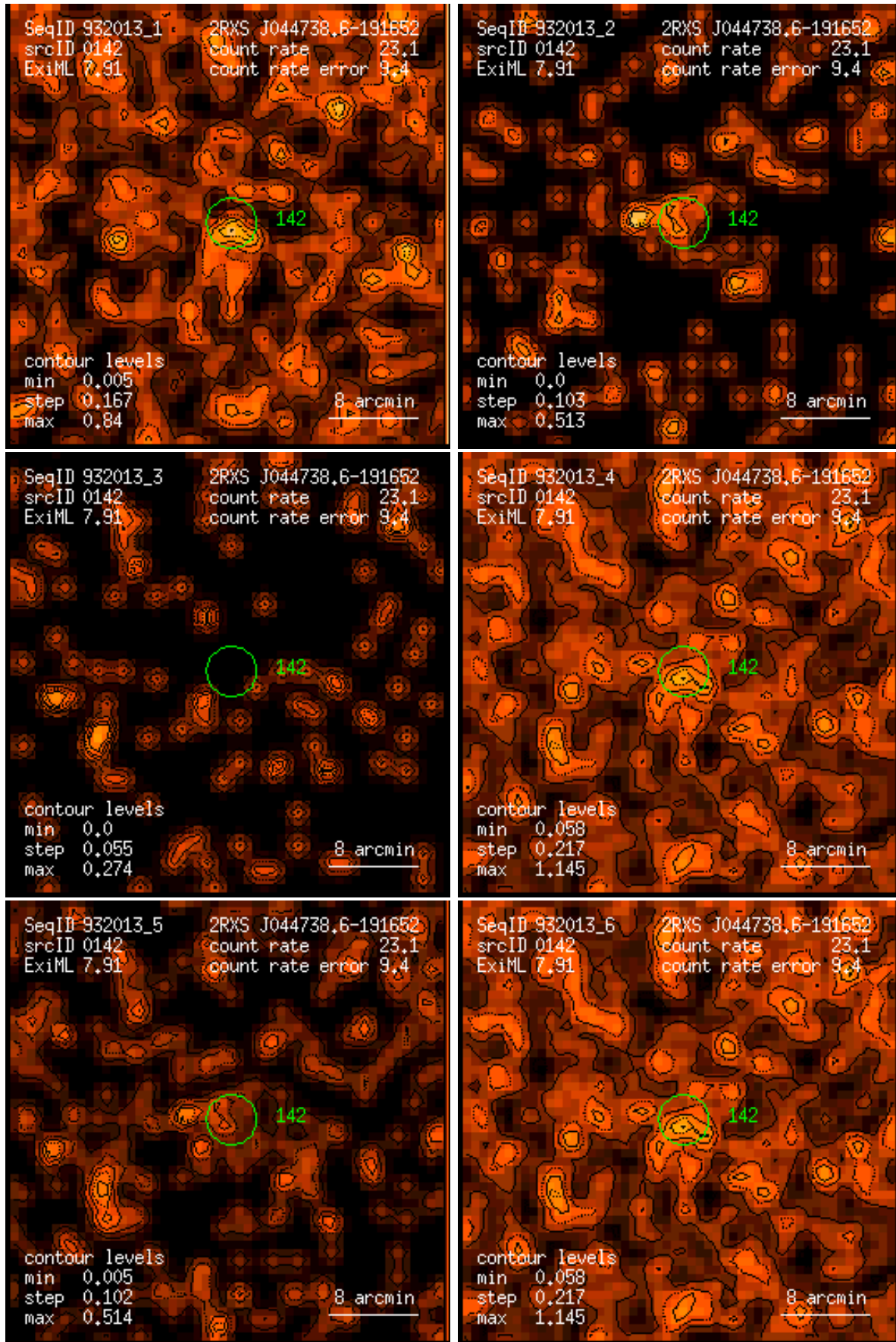
Figure 142: RASS 932013: detection 0142: band rate images, Gaussian filter: (1) PSPC channels 11 – 41, (2) 52 – 90, (3) 91 – 201, (4) 11 – 235, (5) 52 – 201, (6) 11 – 201. Broad band rates in counts/ks. Band rate contour levels in counts/ks/arcmin 2 .
