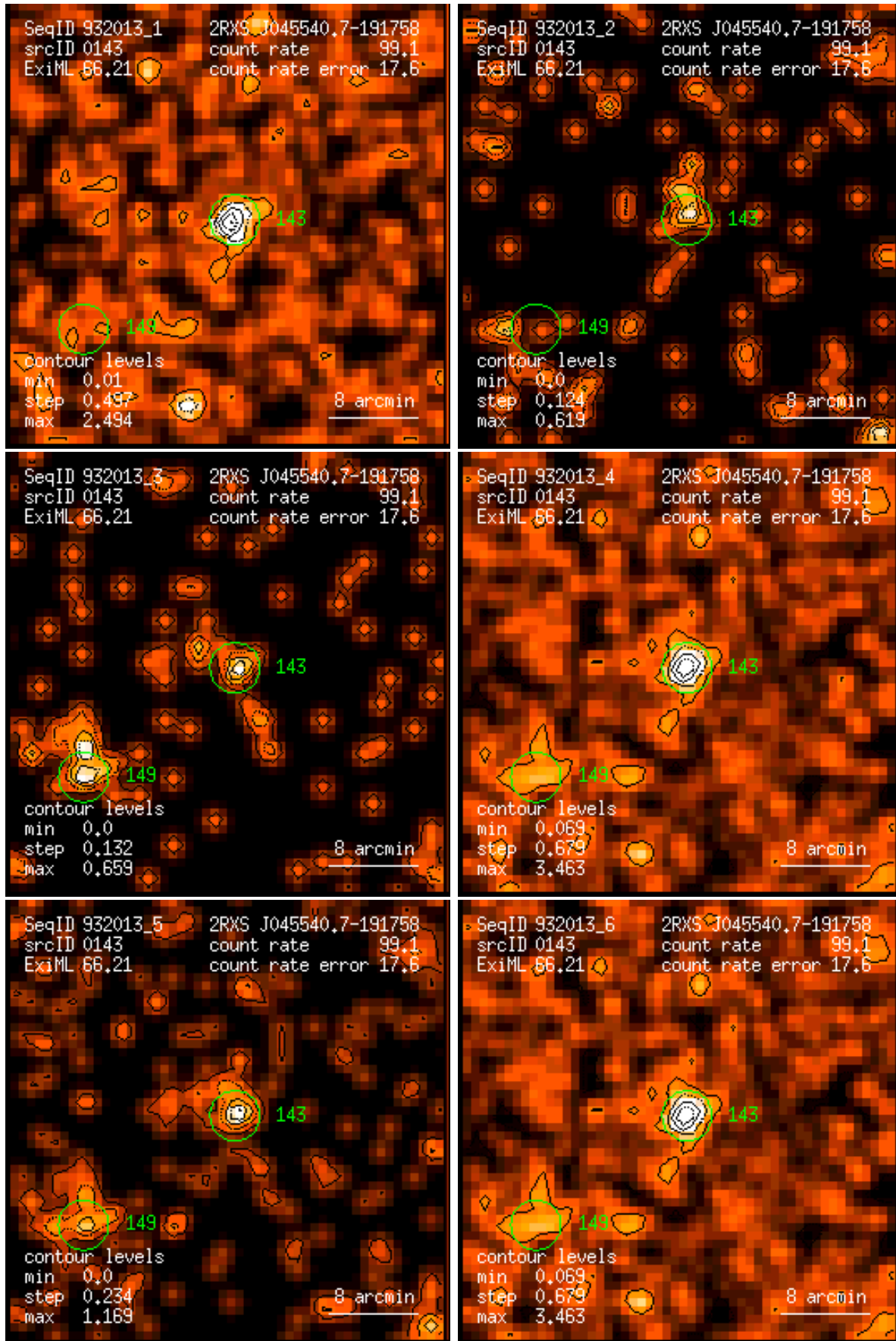
Figure 143: RASS 932013: detection 0143: band rate images, Gaussian filter: (1) PSPC channels 11 – 41, (2) 52 – 90, (3) 91 – 201, (4) 11 – 235, (5) 52 – 201, (6) 11 – 201. Broad band rates in counts/ks. Band rate contour levels in counts/ks/arcmin 2 .
