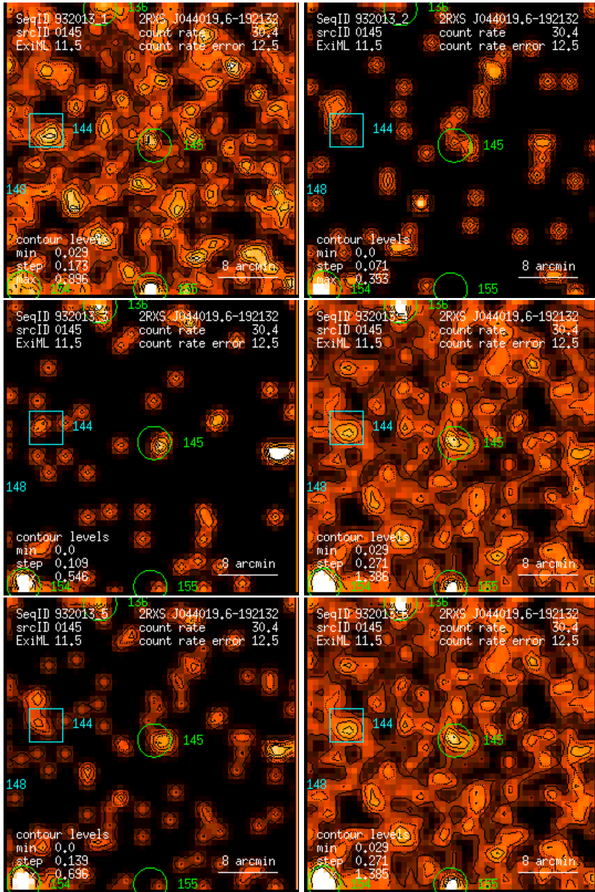
Figure 145: RASS 932013: detection 0145: band rate images, Gaussian filter: (1) PSPC channels 11 – 41, (2) 52 – 90, (3) 91 – 201, (4) 11 – 235, (5) 52 – 201, (6) 11 – 201. Broad band rates in counts/ks. Band rate contour levels in counts/ks/arcmin 2 .
