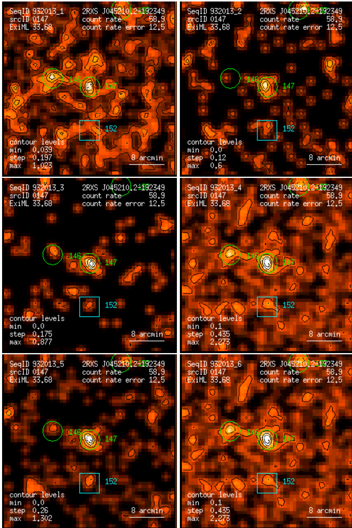
Figure 147: RASS 932013: detection 0147: band rate images, Gaussian filter: (1) PSPC channels 11 – 41, (2) 52 – 90, (3) 91 – 201, (4) 11 – 235, (5) 52 – 201, (6) 11 – 201. Broad band rates in counts/ks. Band rate contour levels in counts/ks/arcmin 2 .
