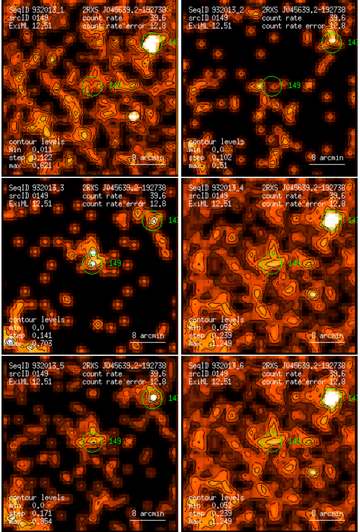
Figure 149: RASS 932013: detection 0149: band rate images, Gaussian filter: (1) PSPC channels 11 – 41, (2) 52 – 90, (3) 91 – 201, (4) 11 – 235, (5) 52 – 201, (6) 11 – 201. Broad band rates in counts/ks. Band rate contour levels in counts/ks/arcmin 2 .
