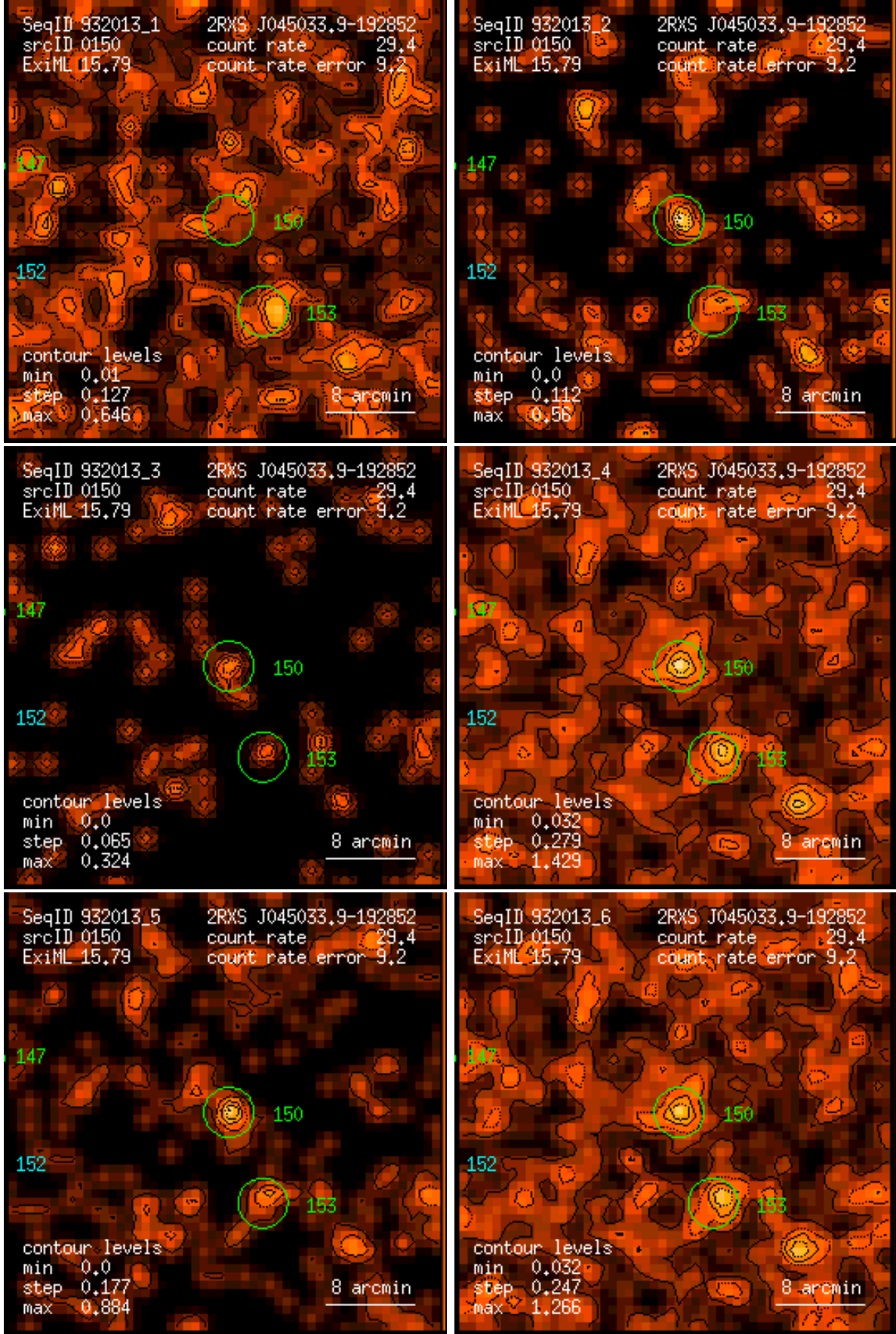
Figure 150: RASS 932013: detection 0150: band rate images, Gaussian filter: (1) PSPC channels 11 – 41, (2) 52 – 90, (3) 91 – 201, (4) 11 – 235, (5) 52 – 201, (6) 11 – 201. Broad band rates in counts/ks. Band rate contour levels in counts/ks/arcmin 2 .
