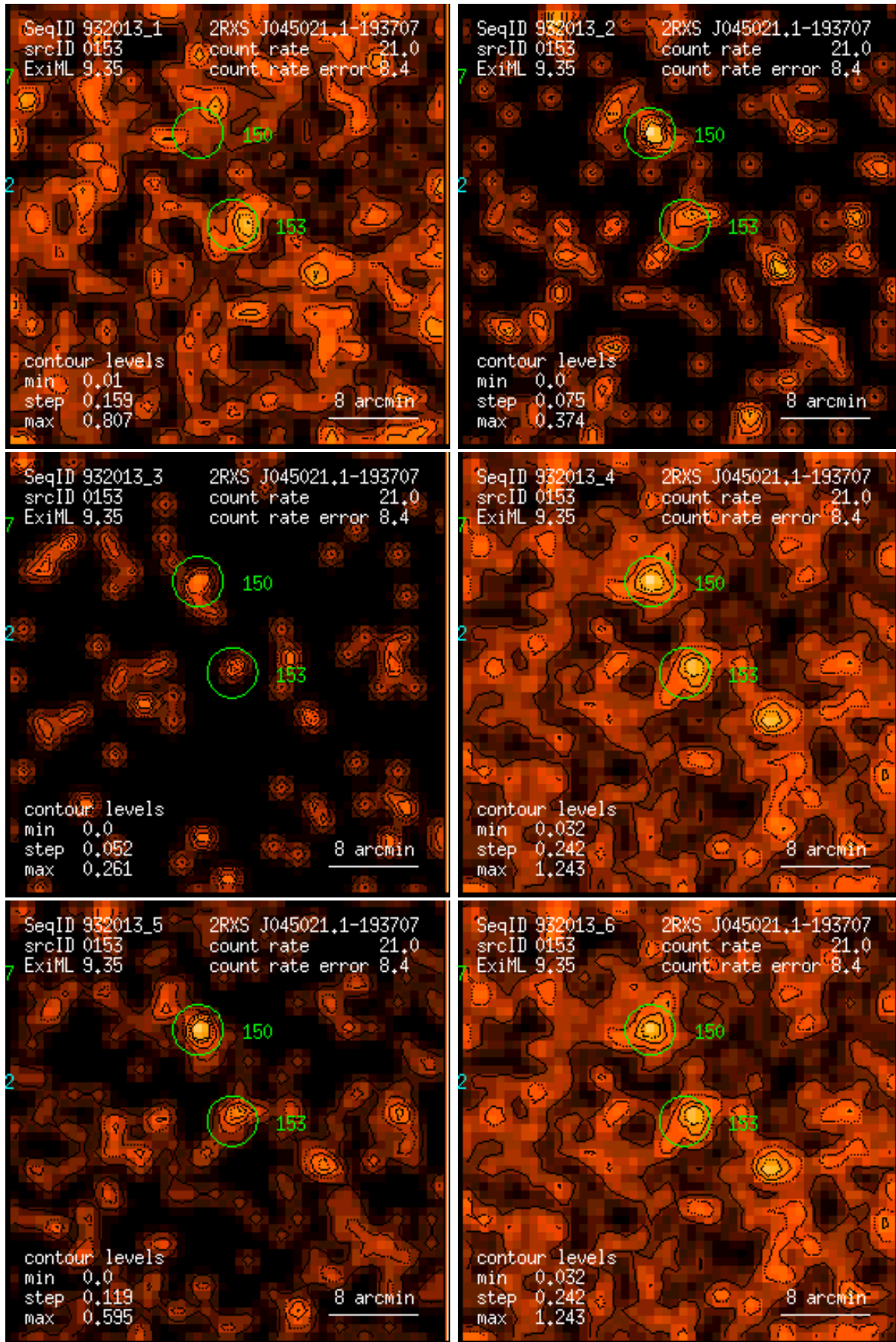
Figure 153: RASS 932013: detection 0153: band rate images, Gaussian filter: (1) PSPC channels 11 – 41, (2) 52 – 90, (3) 91 – 201, (4) 11 – 235, (5) 52 – 201, (6) 11 – 201. Broad band rates in counts/ks. Band rate contour levels in counts/ks/arcmin 2 .
