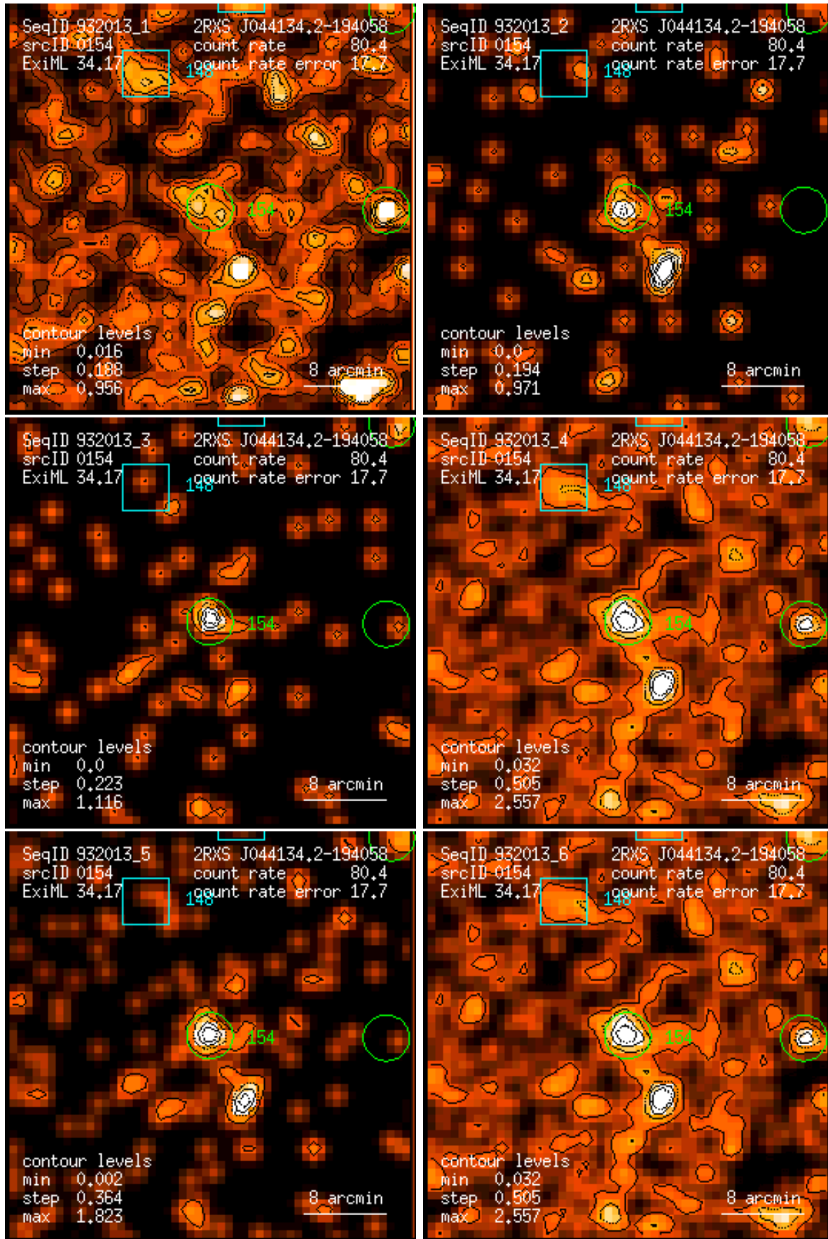
Figure 154: RASS 932013: detection 0154: band rate images, Gaussian filter: (1) PSPC channels 11 – 41, (2) 52 – 90, (3) 91 – 201, (4) 11 – 235, (5) 52 – 201, (6) 11 – 201. Broad band rates in counts/ks. Band rate contour levels in counts/ks/arcmin 2 .
