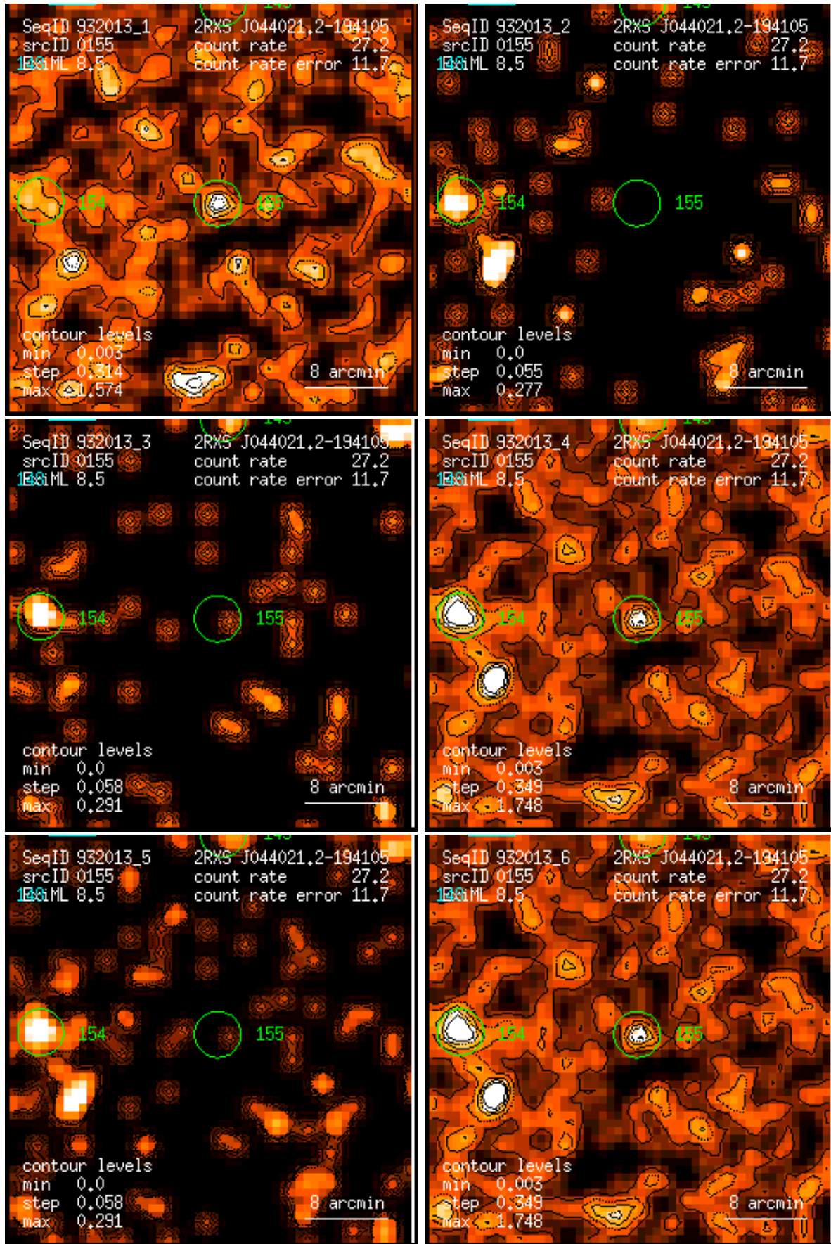
Figure 155: RASS 932013: detection 0155: band rate images, Gaussian filter: (1) PSPC channels 11 – 41, (2) 52 – 90, (3) 91 – 201, (4) 11 – 235, (5) 52 – 201, (6) 11 – 201. Broad band rates in counts/ks. Band rate contour levels in counts/ks/arcmin 2 .
