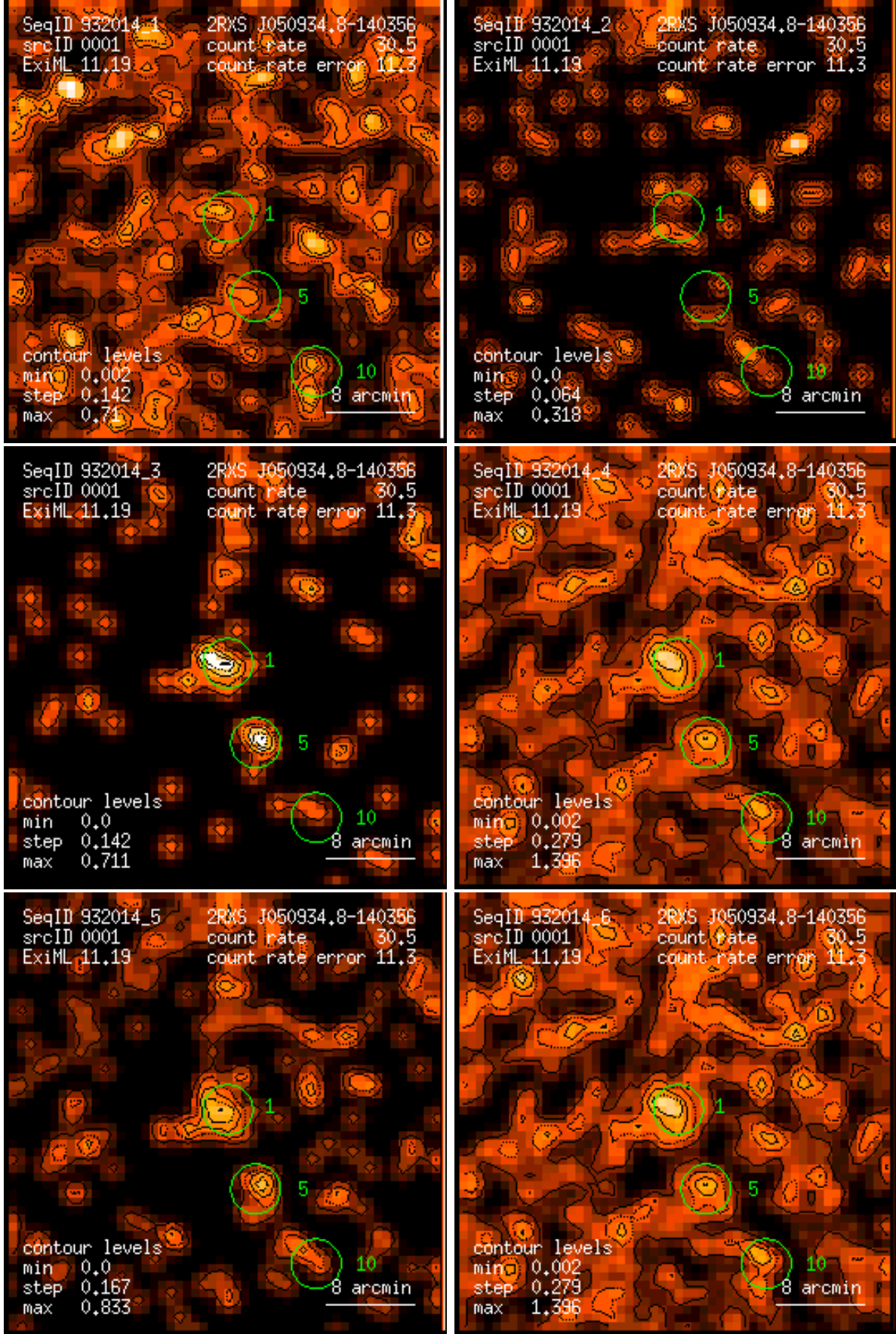
Figure 1: RASS 932014: detection 0001: band rate images, Gaussian filter: (1) PSPC channels 11 – 41, (2) 52 – 90, (3) 91 – 201, (4) 11 – 235, (5) 52 – 201, (6) 11 – 201. Broad band rates in counts/ks. Band rate contour levels in counts/ks/arcmin 2 .
