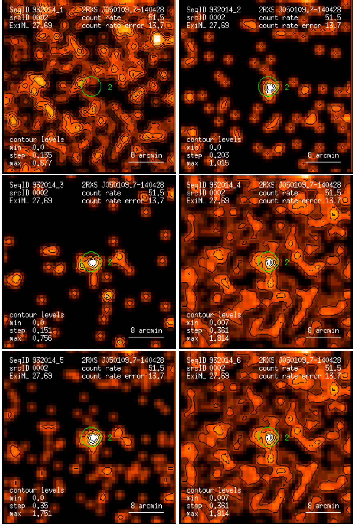
Figure 2: RASS 932014: detection 0002: band rate images, Gaussian filter: (1) PSPC channels 11 – 41, (2) 52 – 90, (3) 91 – 201, (4) 11 – 235, (5) 52 – 201, (6) 11 – 201. Broad band rates in counts/ks. Band rate contour levels in counts/ks/arcmin 2 .
