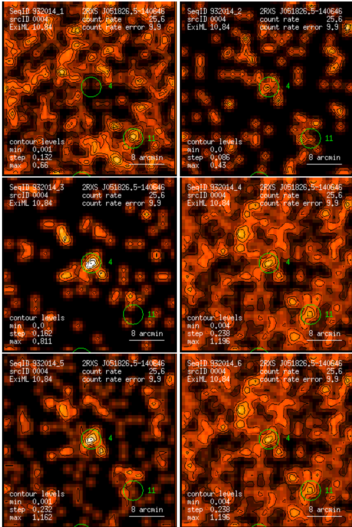
Figure 4: RASS 932014: detection 0004: band rate images, Gaussian filter: (1) PSPC channels 11 – 41, (2) 52 – 90, (3) 91 – 201, (4) 11 – 235, (5) 52 – 201, (6) 11 – 201. Broad band rates in counts/ks. Band rate contour levels in counts/ks/arcmin 2 .
