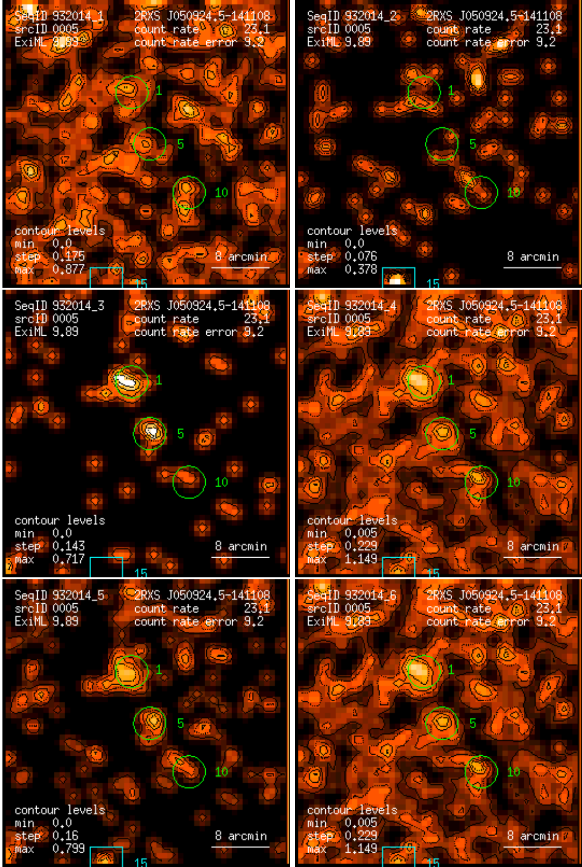
Figure 5: RASS 932014: detection 0005: band rate images, Gaussian filter: (1) PSPC channels 11 – 41, (2) 52 – 90, (3) 91 – 201, (4) 11 – 235, (5) 52 – 201, (6) 11 – 201. Broad band rates in counts/ks. Band rate contour levels in counts/ks/arcmin 2 .
