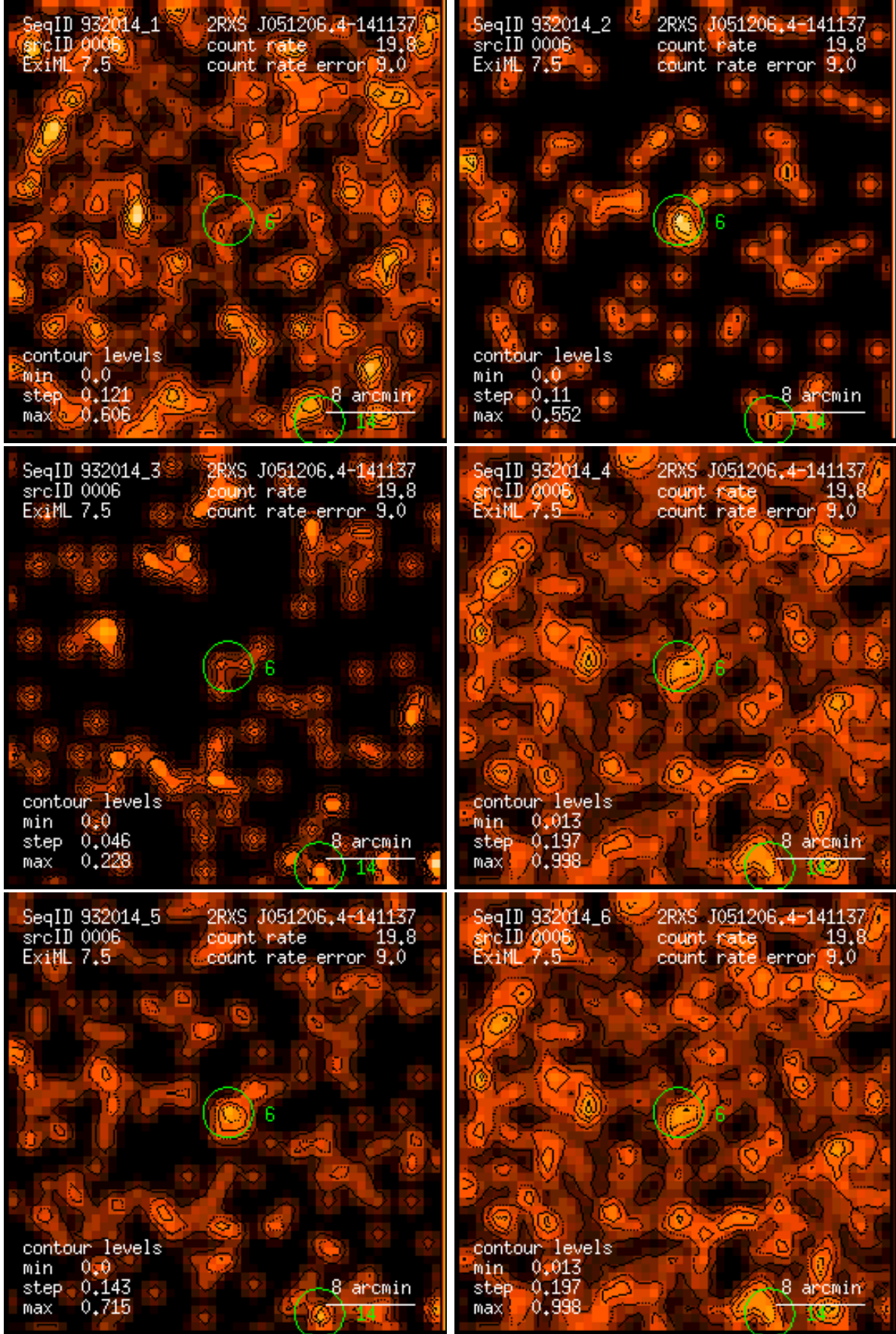
Figure 6: RASS 932014: detection 0006: band rate images, Gaussian filter: (1) PSPC channels 11 – 41, (2) 52 – 90, (3) 91 – 201, (4) 11 – 235, (5) 52 – 201, (6) 11 – 201. Broad band rates in counts/ks. Band rate contour levels in counts/ks/arcmin 2 .
