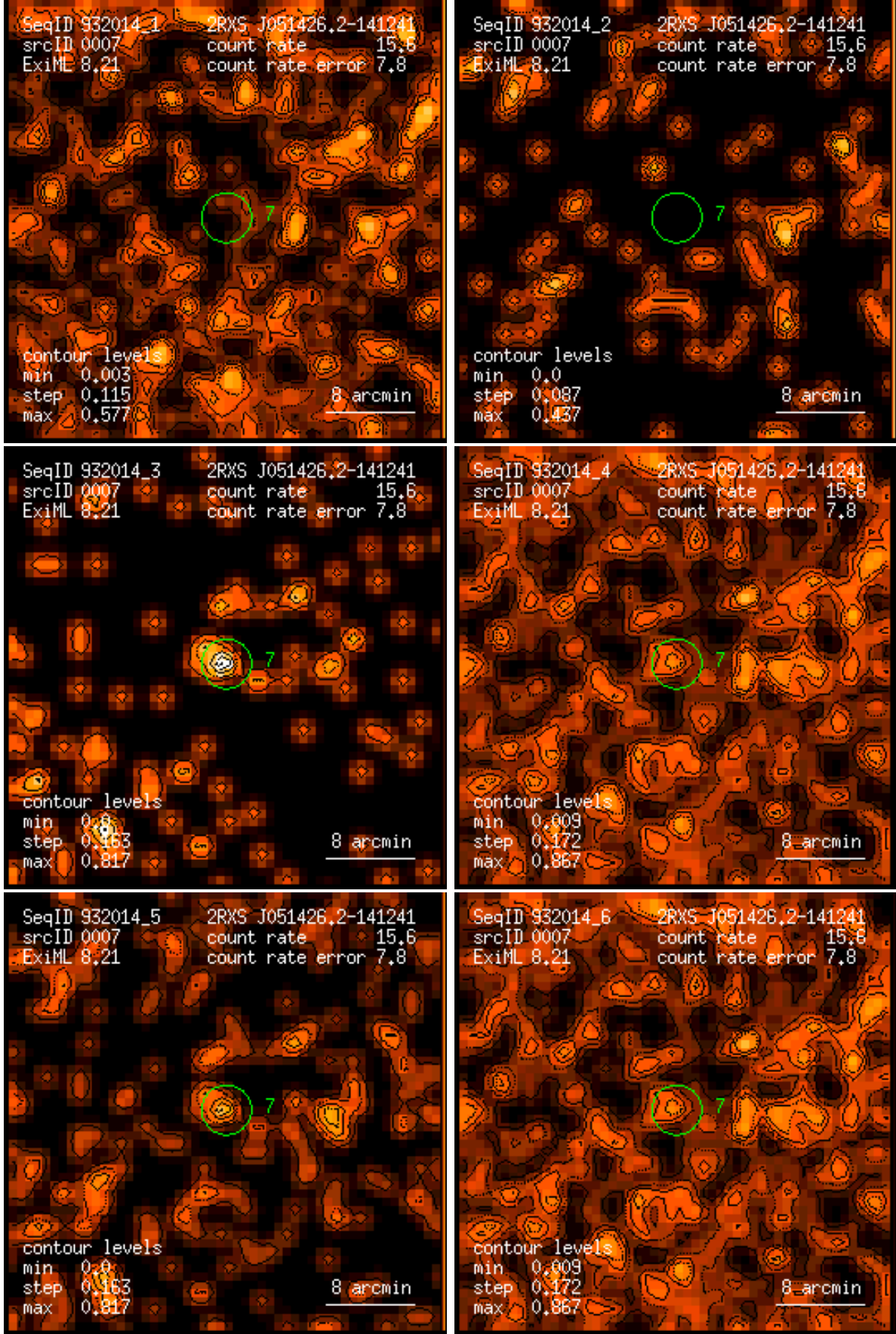
Figure 7: RASS 932014: detection 0007: band rate images, Gaussian filter: (1) PSPC channels 11 – 41, (2) 52 – 90, (3) 91 – 201, (4) 11 – 235, (5) 52 – 201, (6) 11 – 201. Broad band rates in counts/ks. Band rate contour levels in counts/ks/arcmin 2 .
