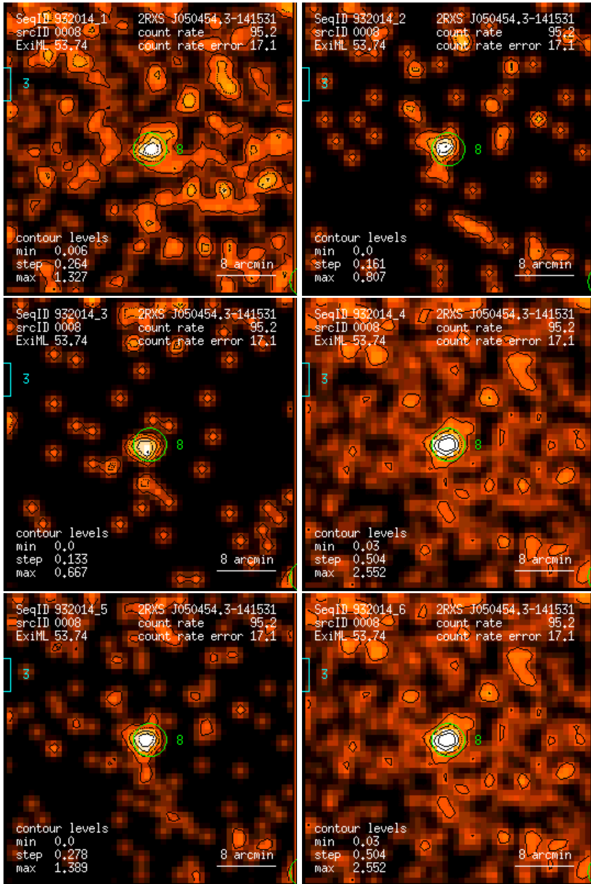
Figure 8: RASS 932014: detection 0008: band rate images, Gaussian filter: (1) PSPC channels 11 – 41, (2) 52 – 90, (3) 91 – 201, (4) 11 – 235, (5) 52 – 201, (6) 11 – 201. Broad band rates in counts/ks. Band rate contour levels in counts/ks/arcmin 2 .
