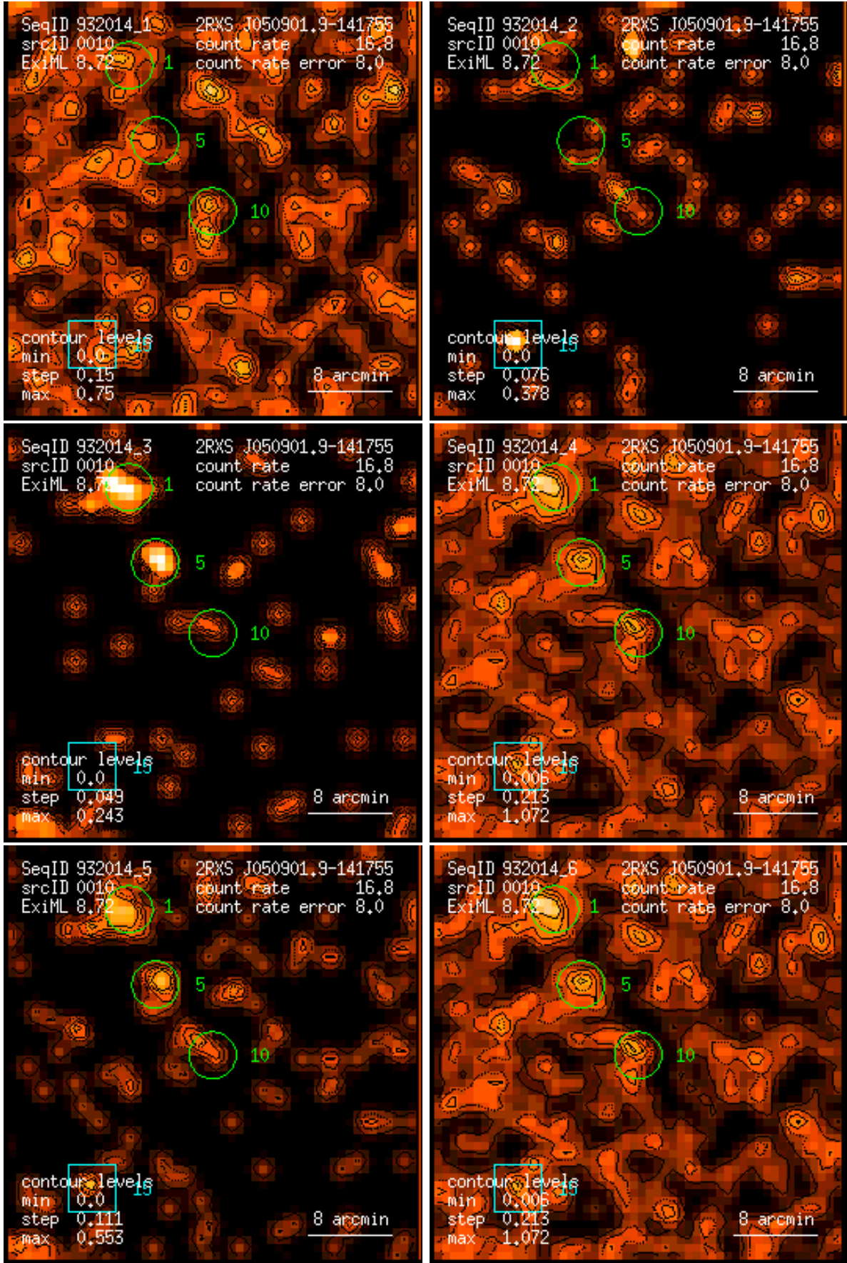
Figure 10: RASS 932014: detection 0010: band rate images, Gaussian filter: (1) PSPC channels 11 – 41, (2) 52 – 90, (3) 91 – 201, (4) 11 – 235, (5) 52 – 201, (6) 11 – 201. Broad band rates in counts/ks. Band rate contour levels in counts/ks/arcmin 2 .
