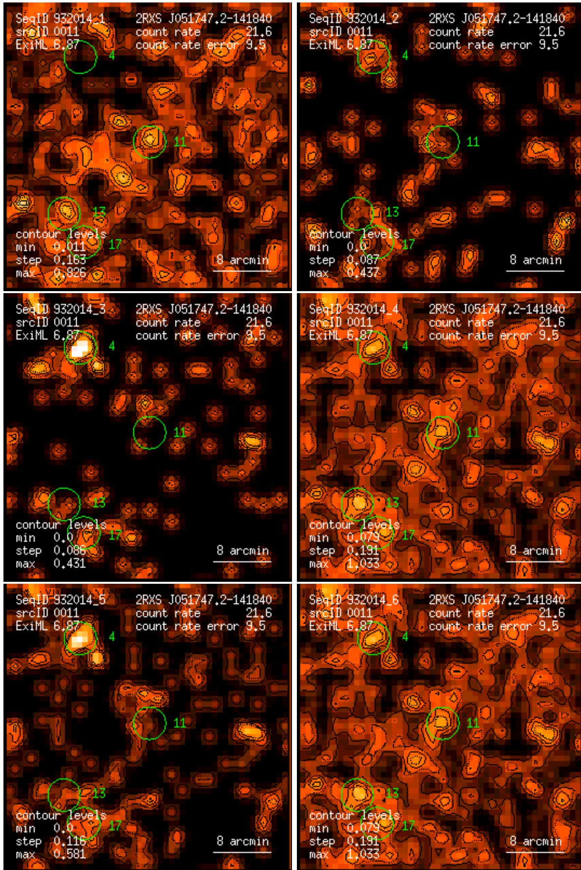
Figure 11: RASS 932014: detection 0011: band rate images, Gaussian filter: (1) PSPC channels 11 – 41, (2) 52 – 90, (3) 91 – 201, (4) 11 – 235, (5) 52 – 201, (6) 11 – 201. Broad band rates in counts/ks. Band rate contour levels in counts/ks/arcmin 2 .
