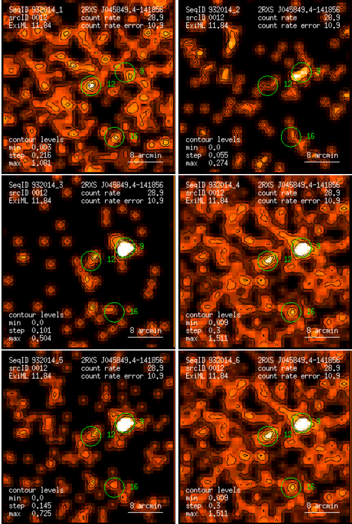
Figure 12: RASS 932014: detection 0012: band rate images, Gaussian filter: (1) PSPC channels 11 – 41, (2) 52 – 90, (3) 91 – 201, (4) 11 – 235, (5) 52 – 201, (6) 11 – 201. Broad band rates in counts/ks. Band rate contour levels in counts/ks/arcmin 2 .
