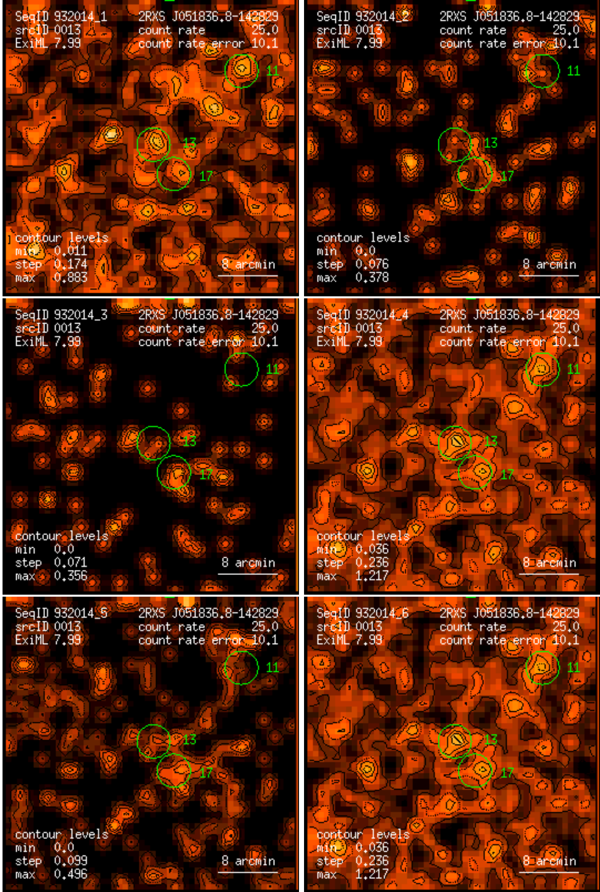
Figure 13: RASS 932014: detection 0013: band rate images, Gaussian filter: (1) PSPC channels 11 – 41, (2) 52 – 90, (3) 91 – 201, (4) 11 – 235, (5) 52 – 201, (6) 11 – 201. Broad band rates in counts/ks. Band rate contour levels in counts/ks/arcmin 2 .
