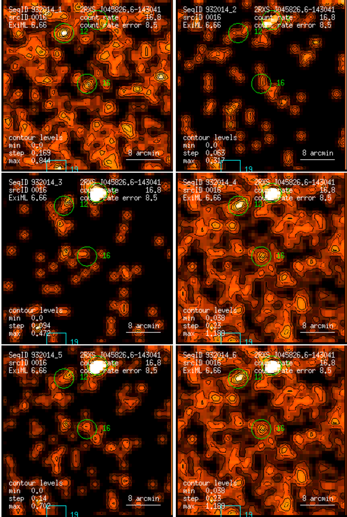
Figure 16: RASS 932014: detection 0016: band rate images, Gaussian filter: (1) PSPC channels 11 – 41, (2) 52 – 90, (3) 91 – 201, (4) 11 – 235, (5) 52 – 201, (6) 11 – 201. Broad band rates in counts/ks. Band rate contour levels in counts/ks/arcmin 2 .
