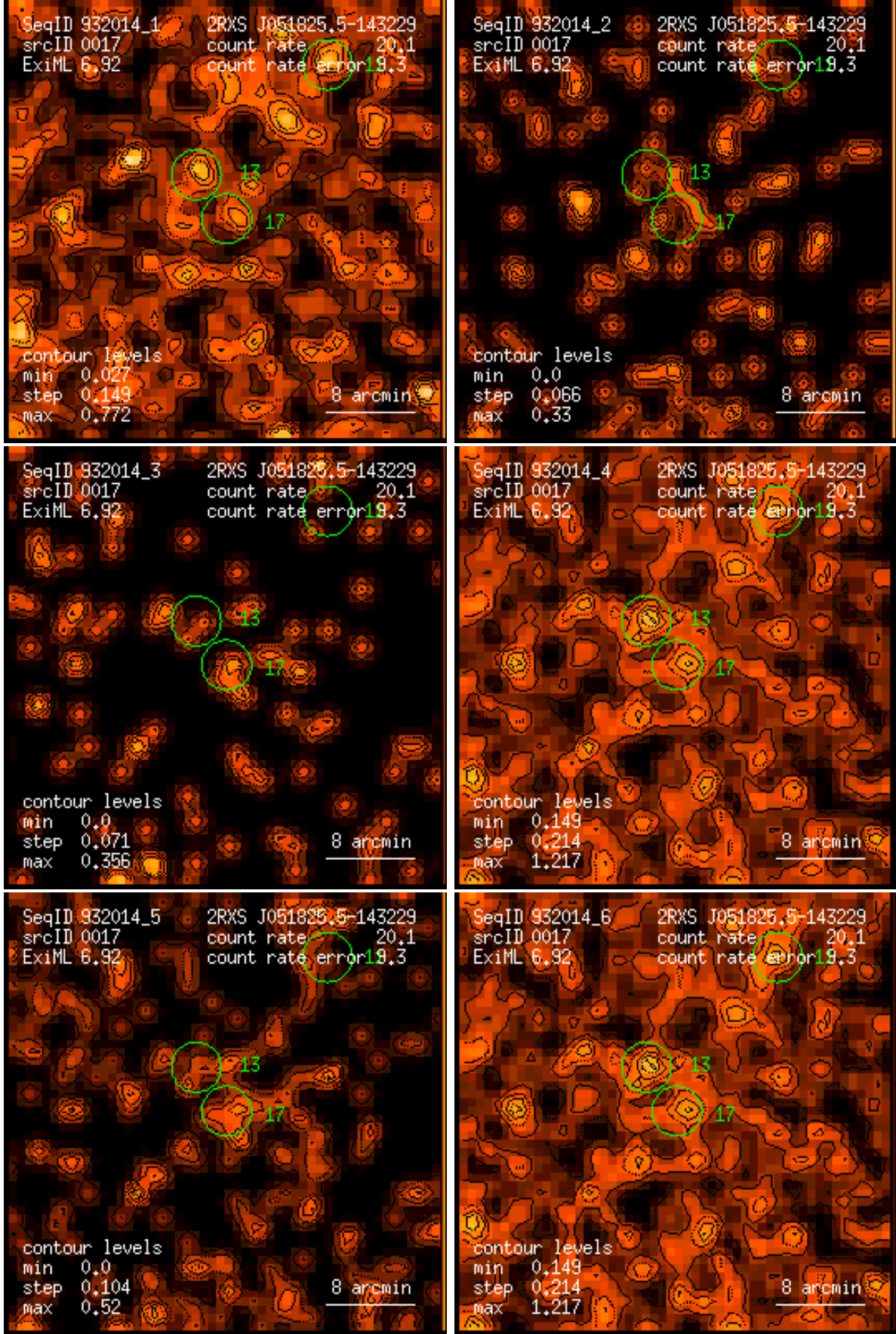
Figure 17: RASS 932014: detection 0017: band rate images, Gaussian filter: (1) PSPC channels 11 – 41, (2) 52 – 90, (3) 91 – 201, (4) 11 – 235, (5) 52 – 201, (6) 11 – 201. Broad band rates in counts/ks. Band rate contour levels in counts/ks/arcmin 2 .
