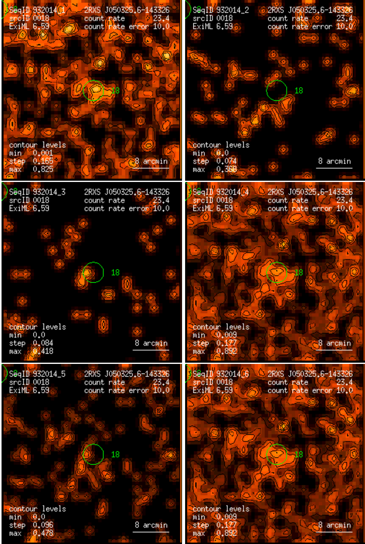
Figure 18: RASS 932014: detection 0018: band rate images, Gaussian filter: (1) PSPC channels 11 – 41, (2) 52 – 90, (3) 91 – 201, (4) 11 – 235, (5) 52 – 201, (6) 11 – 201. Broad band rates in counts/ks. Band rate contour levels in counts/ks/arcmin 2 .
